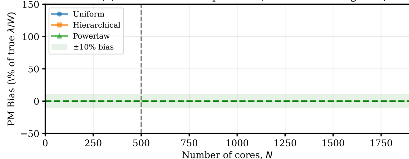
Panel (d): PM Bias vs Sample Size (Smooth Convergence)
