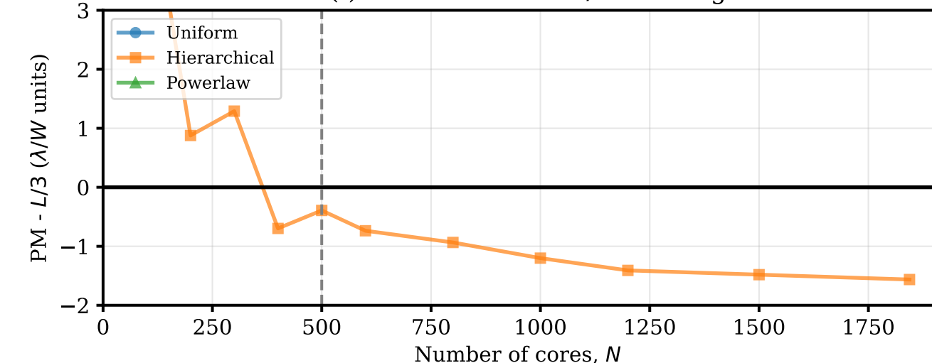
Panel (f): Deviation from L/3 Convergence
