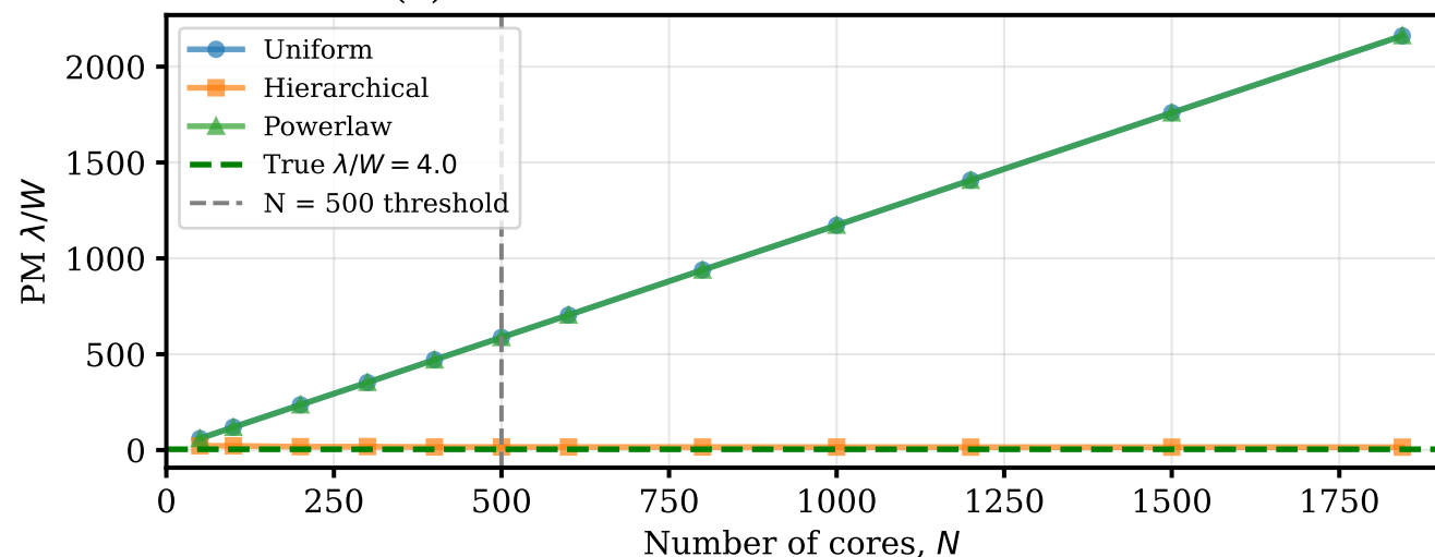
Panel (a): PM Statistic vs N for Different Distributions
