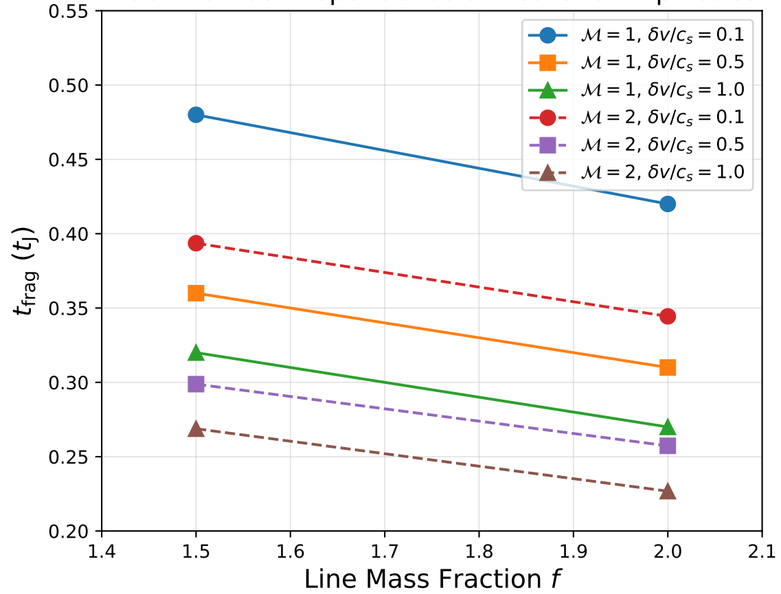
Mach Number Dependence at Realistic Amplitudes
