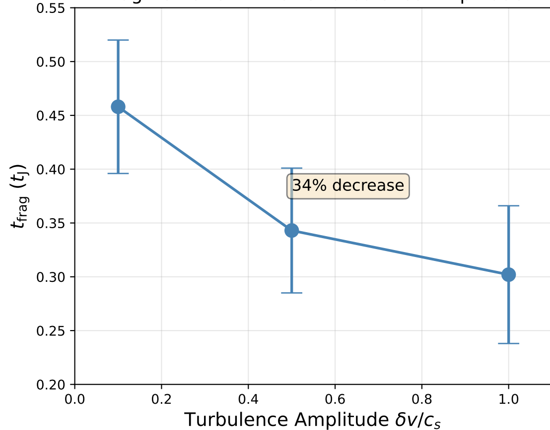
Fragmentation Time vs Turbulence Amplitude
