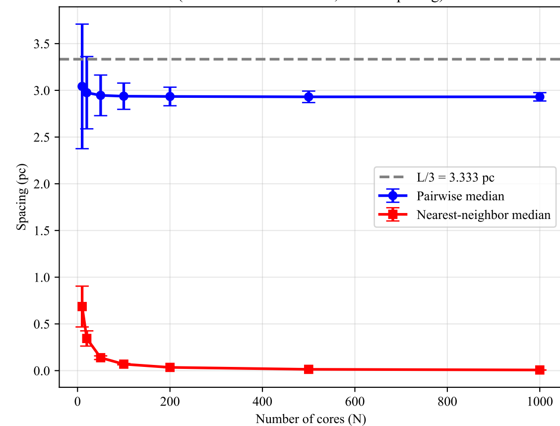
Random/Uniform Distribution (Pairwise median \rightarrow L/3 , no true spacing)
