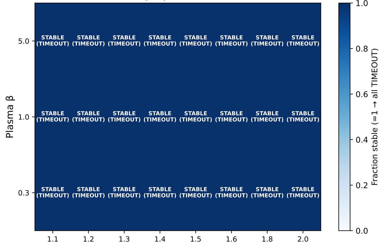
BRIDGE_GRID Stability Map \theta=90^\circ (perpendicular field)
