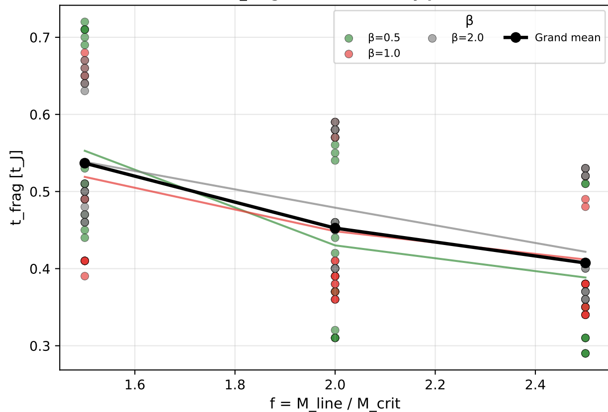
CALIBRATION_VALIDATION (Final) t_{\text{frag}} vs f , coloured by \beta
