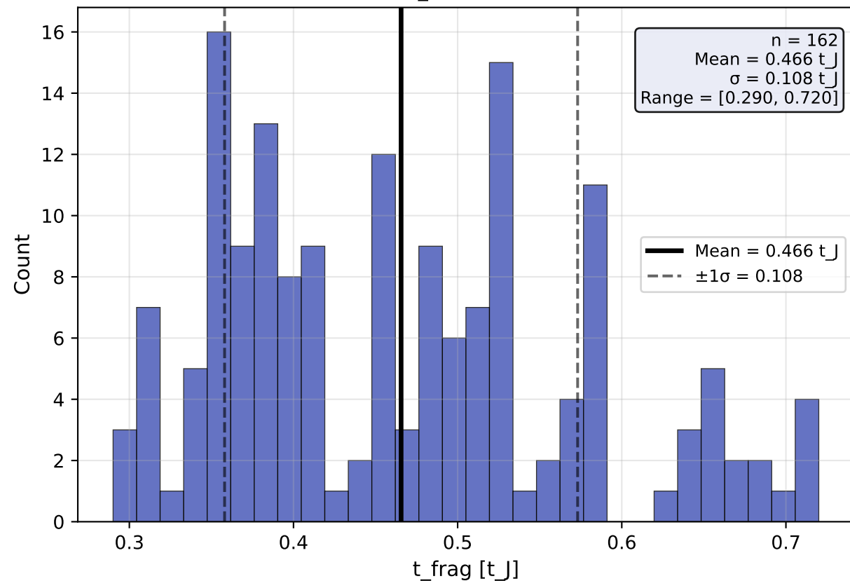
t_{\text{frag}} Distribution CALIBRATION_VALIDATION (n=162)
