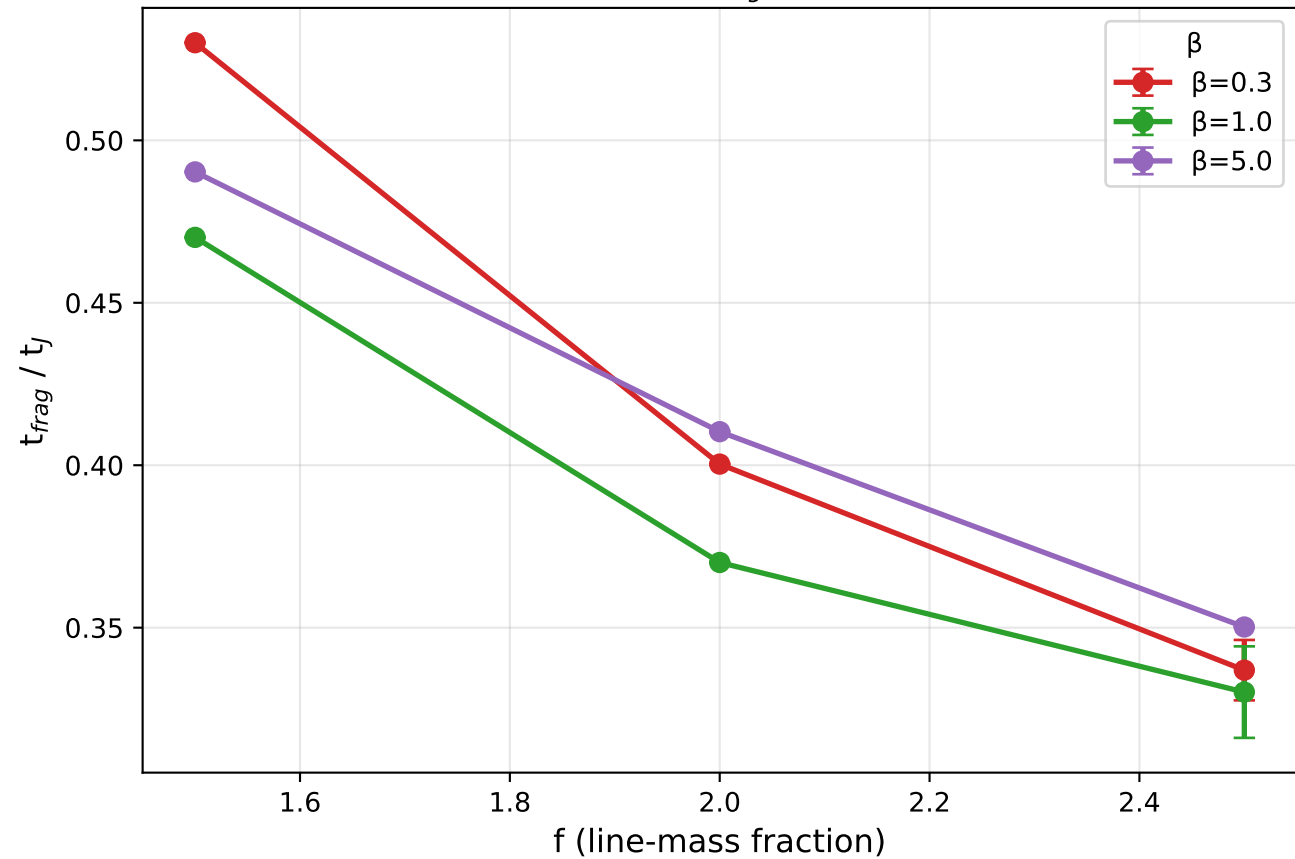
SUPERCRITICAL_LONG: t_{frag} vs Line-Mass Fraction
