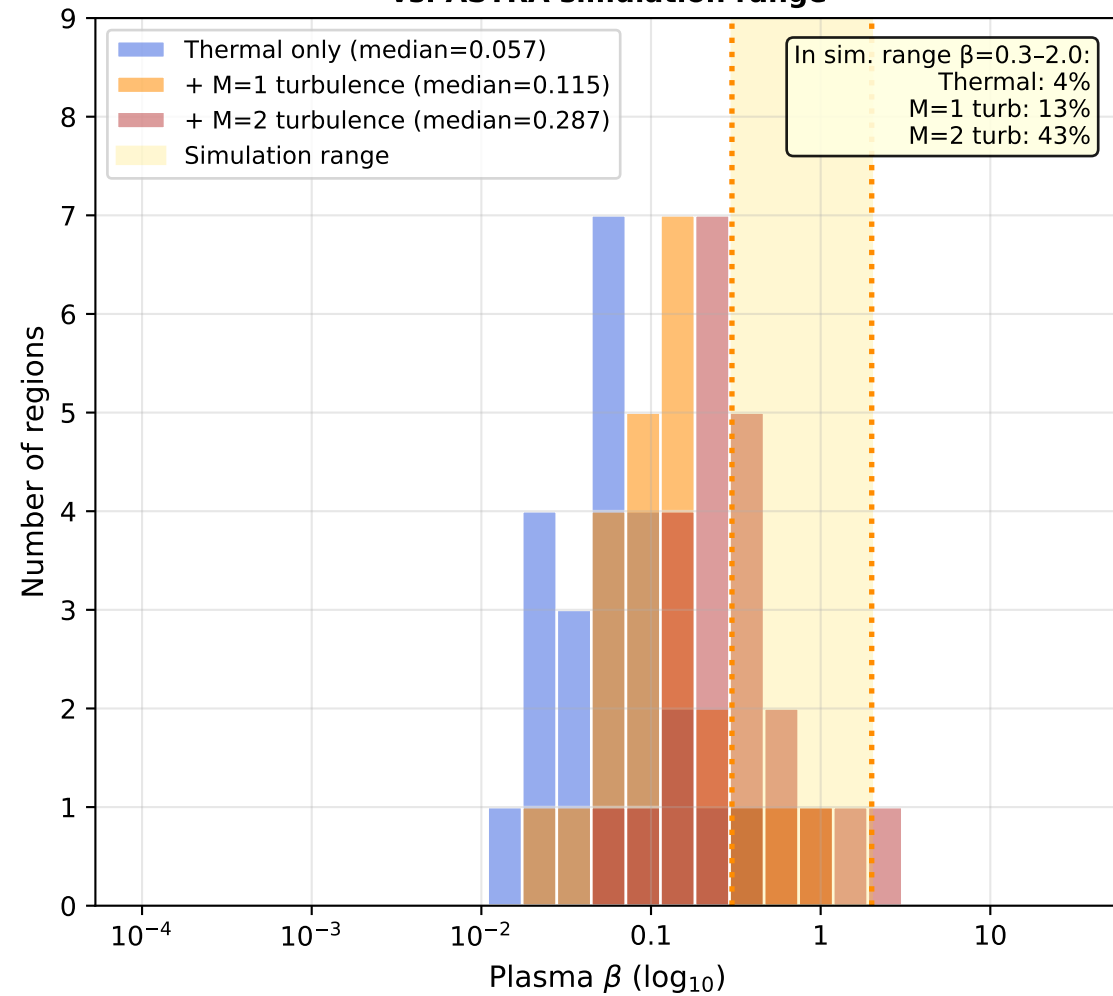
(b) \beta distributions: thermal vs. turbulent-effective vs. ASTRA simulation range
