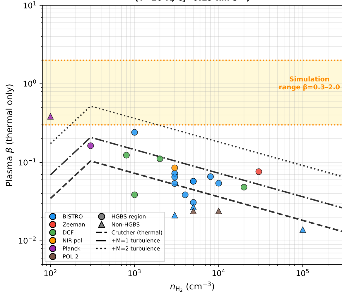
(a) Thermal \beta vs. density in HGBS filaments ( T=10 K, c_s=0.19 km s ^{-1} )
