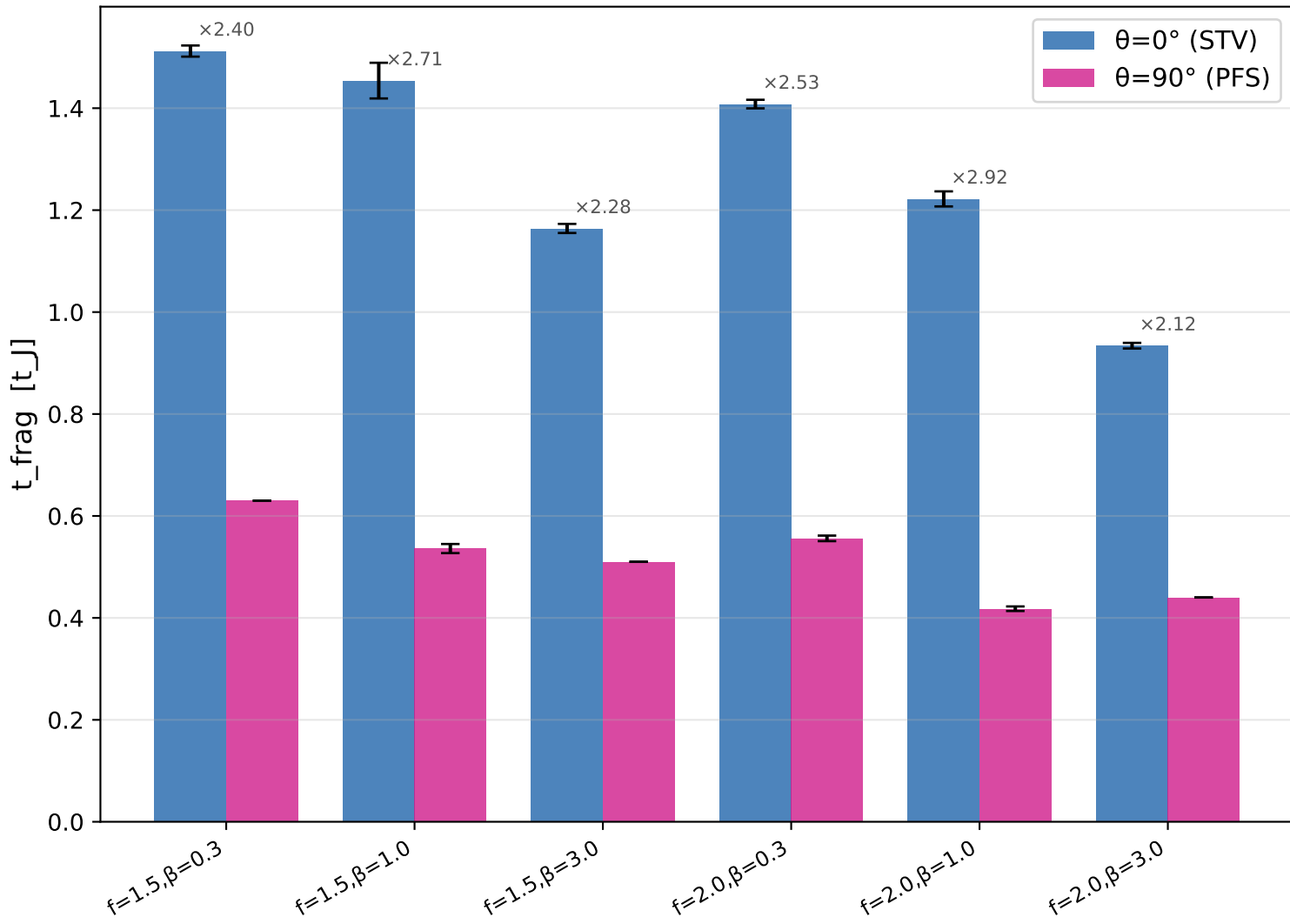
Geometry Effect: \theta=0^\circ vs \theta=90^\circ (matched f , \beta )
