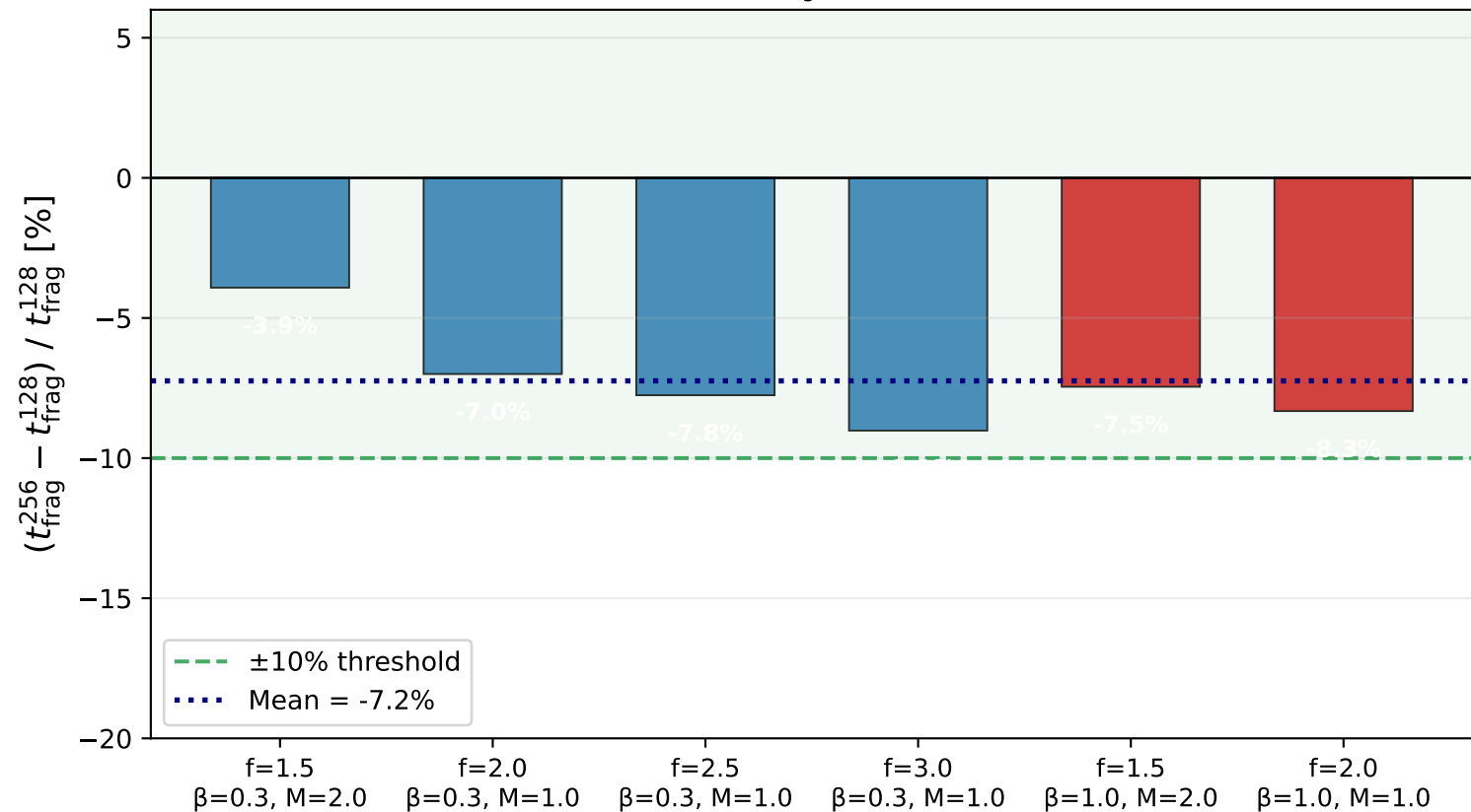
Resolution Effect on t_{\text{frag}} : Percentage Difference
