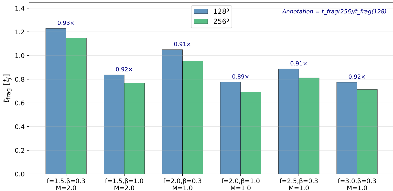
Resolution Comparison: t_{\text{frag}} at 128^3 vs 256^3 (both using athena_pr PRR pgen)
