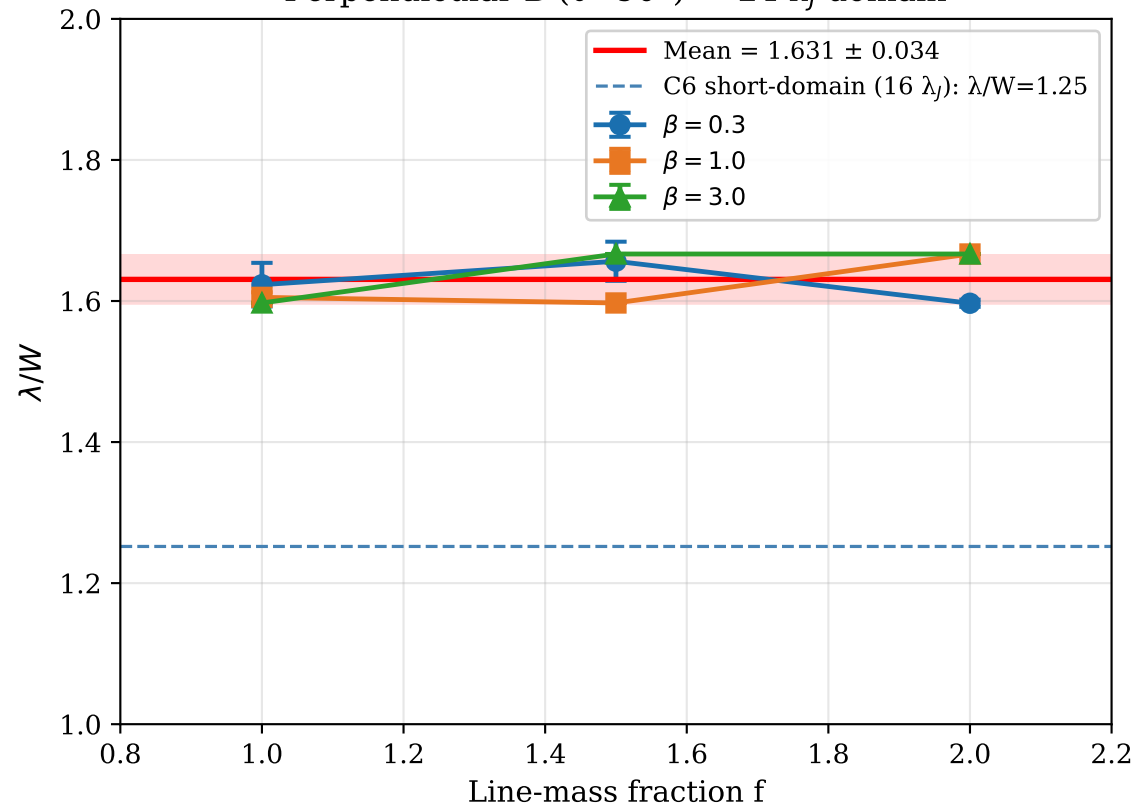
Perpendicular B ( \theta=90^\circ ) — 24 \lambda_J domain
