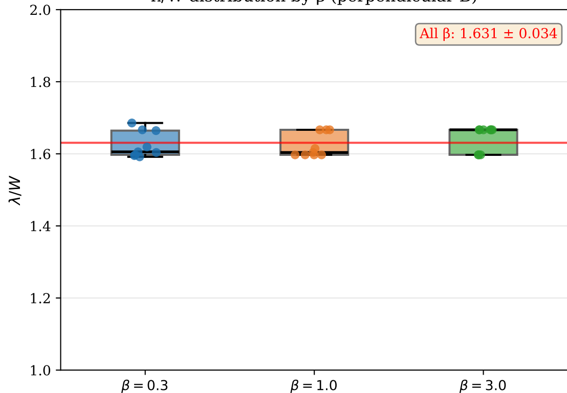
\lambda/W distribution by \beta (perpendicular B)
