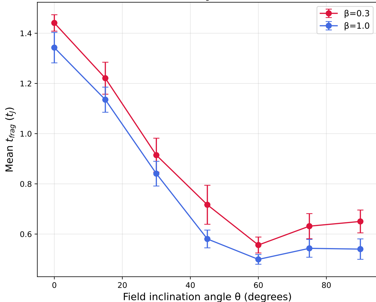
Campaign A: t_{frag}(\theta) by plasma- \beta
