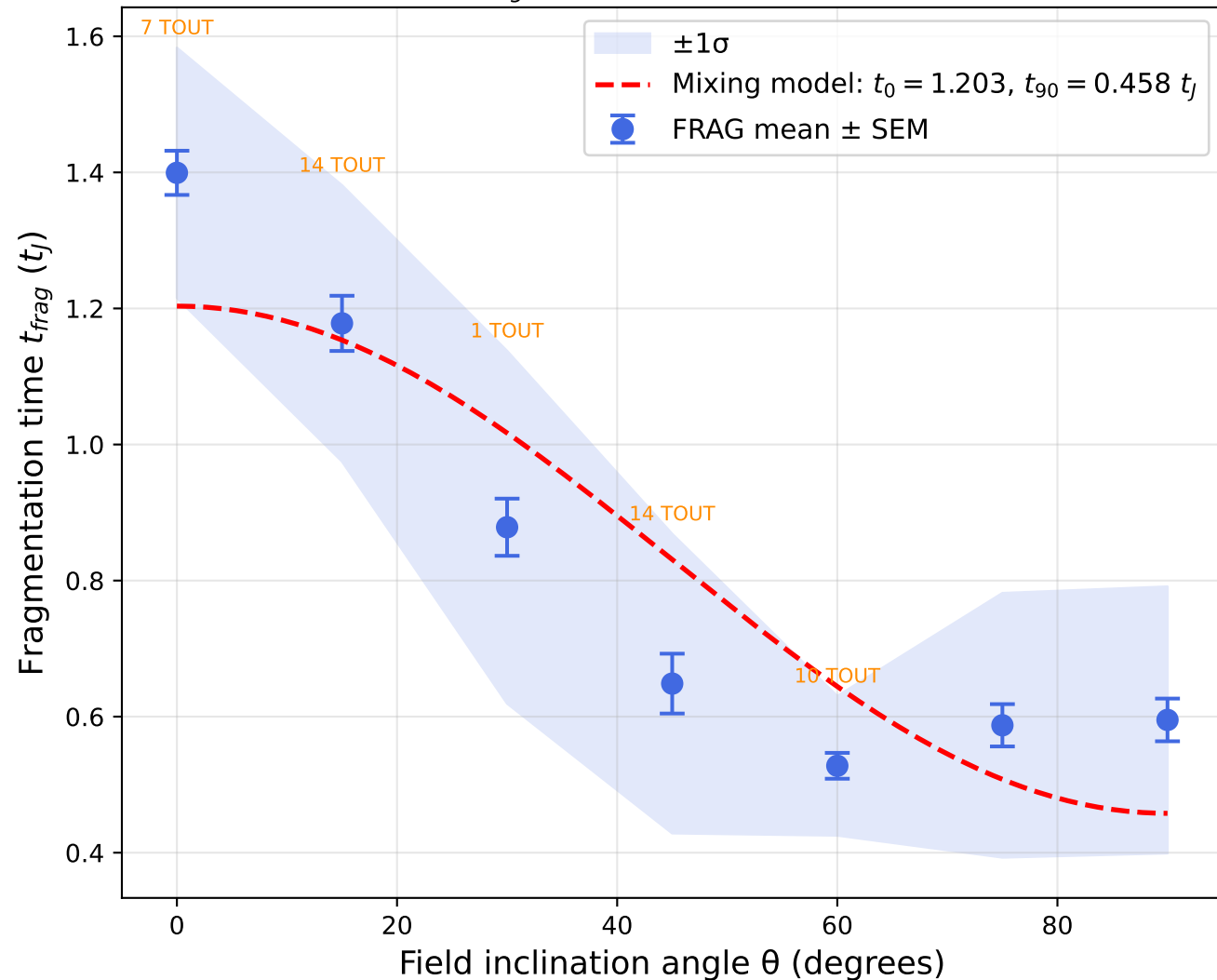
Campaign A: t_{frag}(\theta) — Field Geometry Mixing Model
