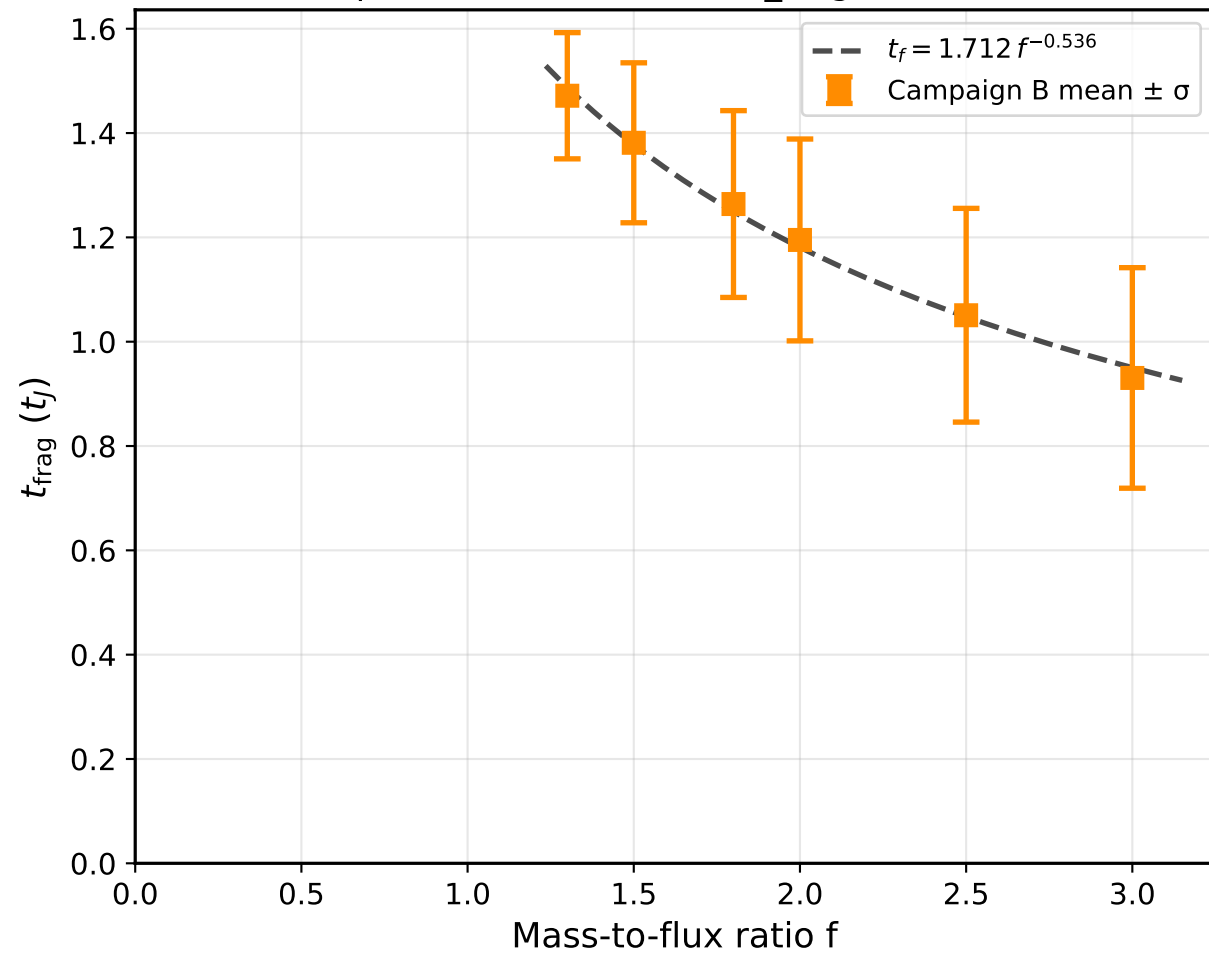
Supercritical Calibration: t_{\text{frag}}(f) at \theta=0^\circ
