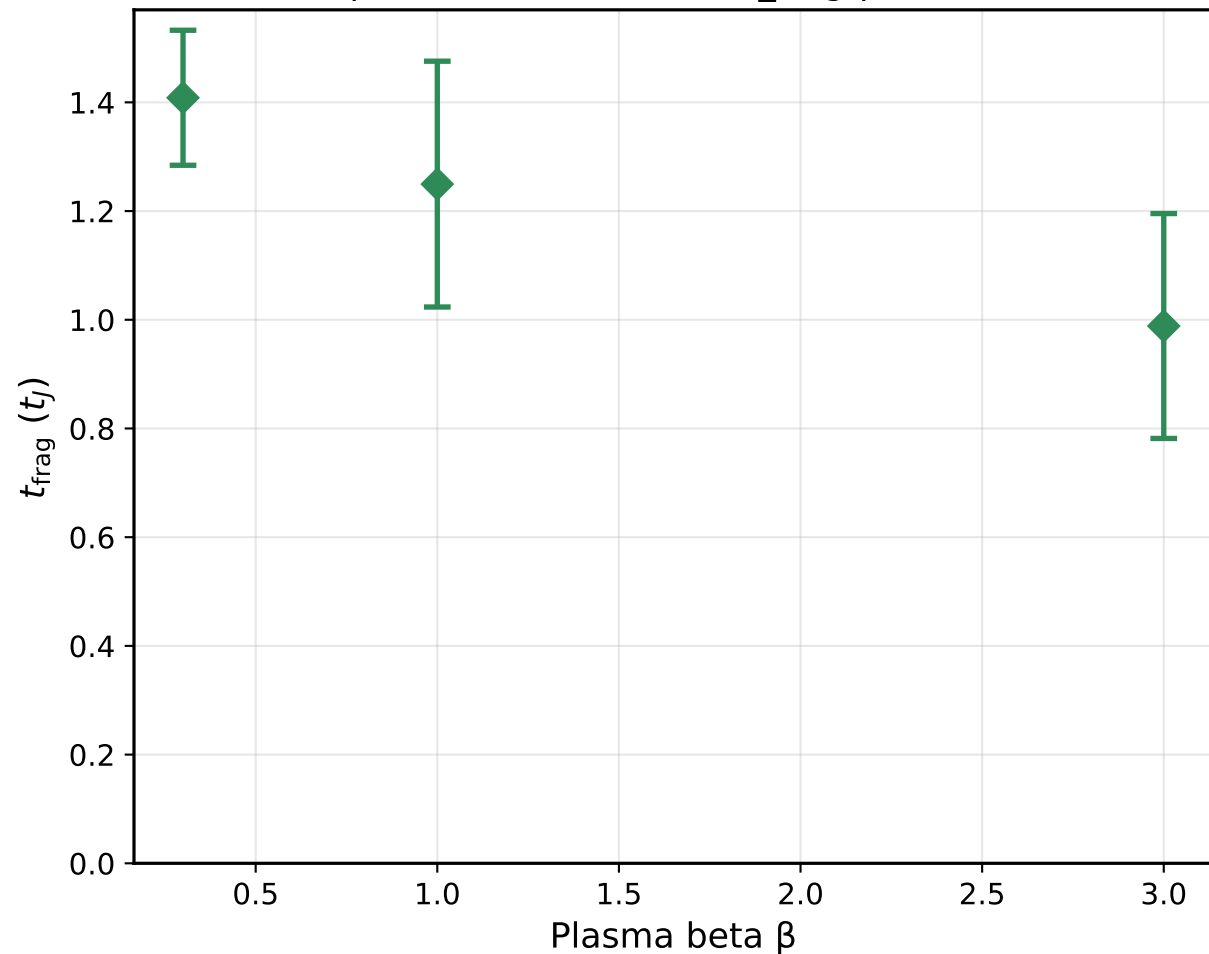
Supercritical Calibration: t_{\text{frag}}(\beta) at \theta=0^\circ
