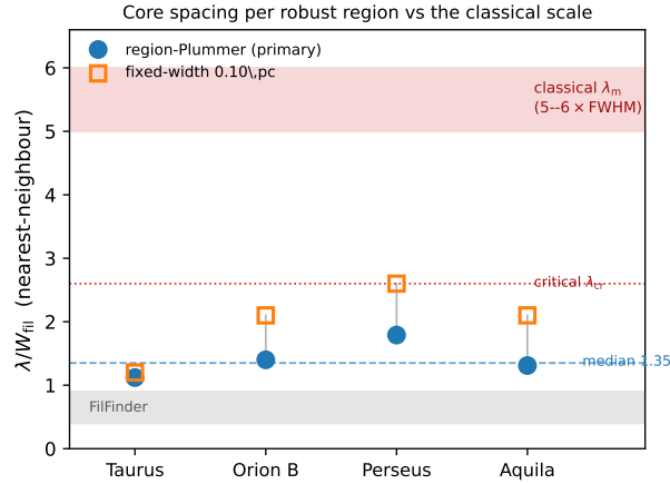
Figure 2. Primary nearest-neighbour core spacing \lambda/W_{\text{fil}} per robust region, in the two DisPerSE width conventions: directly-measured region-Plummer widths (blue circles, our primary; per-region raw 1.12, 1.40, 1.79, 1.31, median 1.35, dashed) and the fixed 0.10 pc width (orange squares; 1.2, 2.1, 2.6, 2.1), both shown raw (before the uniform injection–recovery correction, which lowers them; Section 2.7). The red band is the classical fastest-growing wavelength \lambda_m \approx 5\text{--}6 \times \text{FWHM} (Fischera & Martin 2012; = 4 \times the flat diameter, Inutsuka & Miyama 1992), and the dotted line the classical critical wavelength \lambda_{\text{cr}} \approx 2.6 \times \text{FWHM} ; every region lies well below both. The grey band marks the independent FilFinder skeleton range ( \lambda/W \approx 0.4\text{--}0.9 ). The deficit is sub-classical in sign under every convention; its magnitude is dominated by the width/skeleton choice, not statistical error (Section 2.9).
