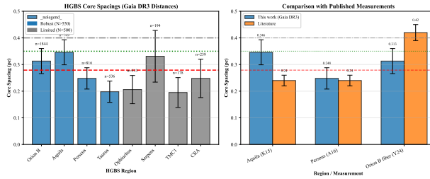
Figure 2. Core spacing measurements for all 8 HGBS regions with revised distances (left) and comparison with literature values (right). Left: per-region spacing with standard-error bars, showing the legacy pairwise-median ( L/3 extent-scale) values retained only for comparison with older work — not the primary nearest-neighbour measure (Section 2.7). Horizontal lines mark the weighted mean (0.279 pc, dashed) and the IM92 prediction (dash-dotted): the latter is drawn at the often-quoted 4 \times \text{FWHM} = 0.4 pc, whereas the correct classical fastest-growing scale is \lambda_m \approx 5\text{--}6 \times \text{FWHM} = 0.5\text{--}0.6 pc (Section 3). These pairwise-median values are not fragmentation wavelengths (Section 2.6); the primary NN per-region values ( \lambda/W = 1.2, 2.1, 2.6, 2.1 ) are given in Section 2.7. Right: comparison with published values (grey bars); our measurements (blue) differ from the published values through a combination of the Gaia DR3 distance revisions (large for Aquila/Serpens) and the homogeneous DisPerSE+NN re-analysis (which dominates for Orion B, whose distance is essentially unchanged), so the shift is not uniform (Taurus decreases slightly).
