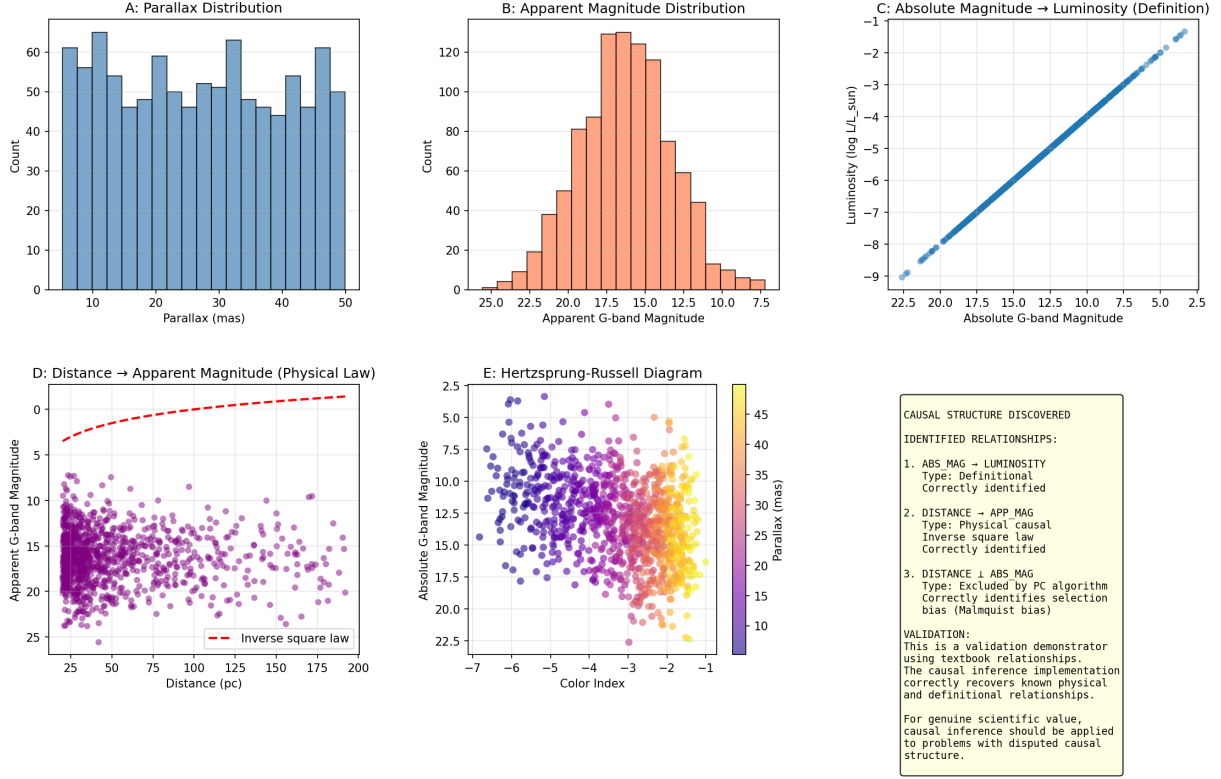
Figure 5. Causal inference analysis of 1,000 Gaia DR2 stars. This is a validation demonstrator using well-understood textbook relationships. ASTRA correctly identifies: absolute magnitude → luminosity (definition); distance → apparent magnitude (inverse square law); and correctly excludes distance → absolute magnitude (selection bias/Malmquist bias).
