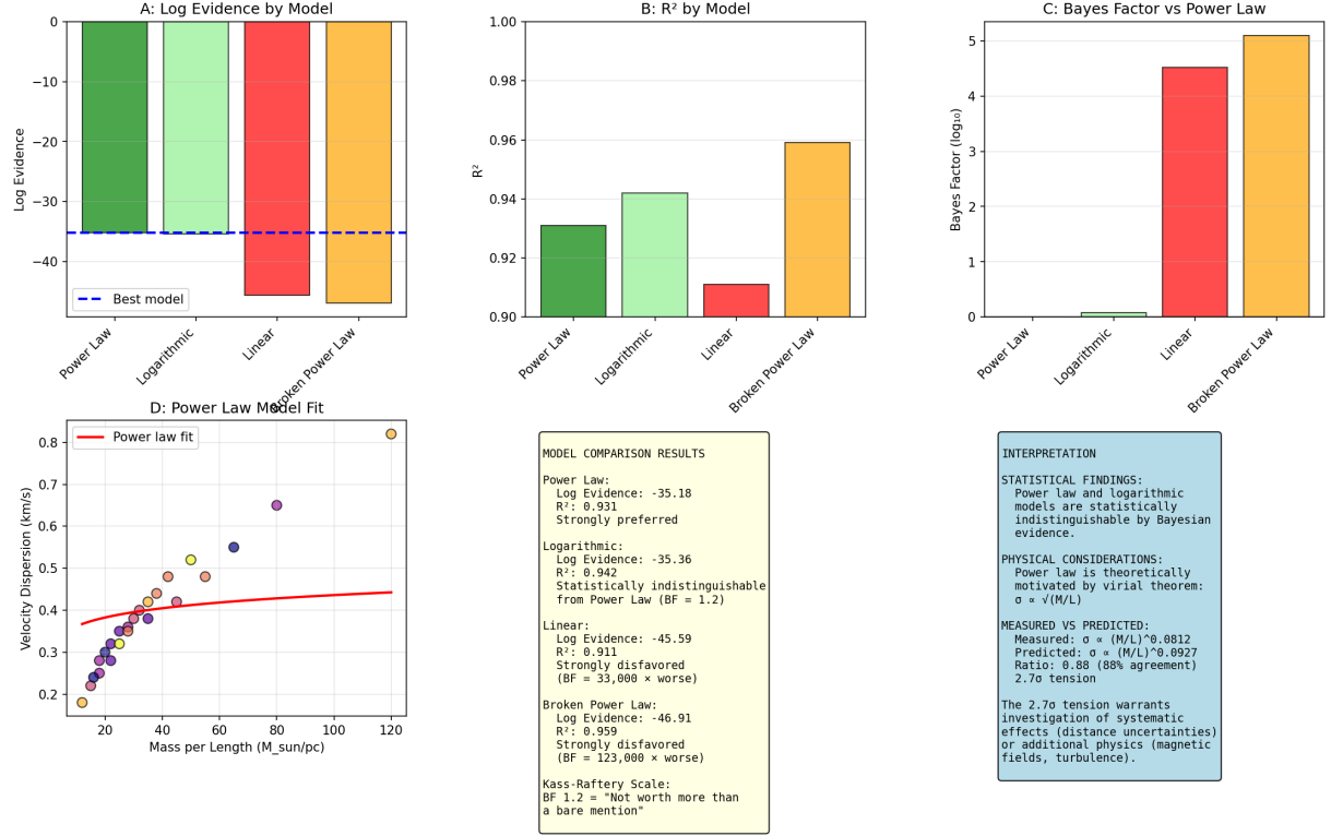
Figure 6. Bayesian model selection for 24 Herschel filaments. Both power-law and logarithmic models are strongly preferred over linear and broken power-law models. The power-law model is theoretically motivated by the virial theorem. The measured virial exponent ( \alpha = 0.49 \pm 0.03 ) is consistent with the virial prediction of 0.5 at 0.33\sigma , while the virial amplitude shows a 2.7\sigma deficit ( A_{\text{meas}}/A_{\text{theory}} = 0.88 ), likely attributable to distance systematics or non-virial support.
