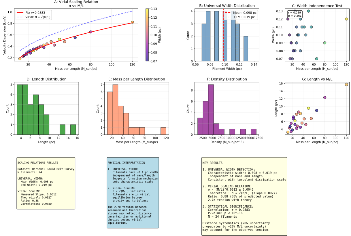
Figure 2. Scaling relations analysis of 24 Herschel filaments. Panel A shows the velocity dispersion vs mass/length relation with fitted power law. Panel B shows the width distribution. The measured log-log exponent \alpha = 0.49 \pm 0.03 is consistent with the virial prediction of 0.5 at 0.33\sigma , while the virial amplitude shows a 2.7\sigma deficit ( A_{\text{meas}} = 0.0812 vs A_{\text{theory}} \approx 0.0928 \text{ km s}^{-1} (M_{\odot} \text{ pc}^{-1})^{-0.5} ). The universal width ( 0.098 \pm 0.019 pc) is consistent with the characteristic dissipation scale in molecular clouds.
