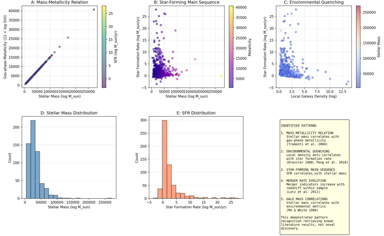
Figure 4. Pattern recognition analysis of 600 SDSS galaxies. ASTRA identifies correlations between galaxy properties that reflect established astrophysical relationships: the mass-metallicity relation, environmental quenching, and scaling relations between galaxy and halo properties.
