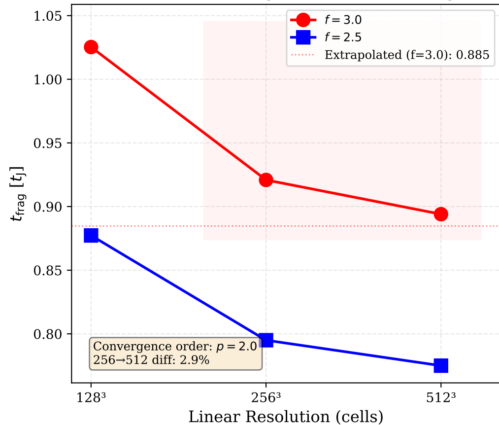
(a) Resolution Convergence ( \beta_c = 0.5 , hourglass)
