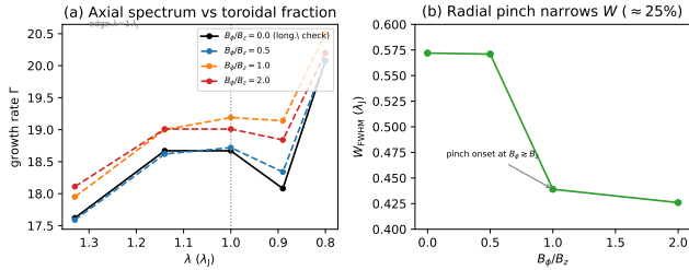
Figure 13. Divergence-free helical-field scan ( B_\phi/B_z = 0 – 2 , 512 \times 128^2 ; Section 4.3). (a) The axial growth-rate spectrum \Gamma(\lambda) in the physical band is invariant to the toroidal fraction ( < 6\% , fit noise), with the converged-band edge fixed at \lambda \approx 1 \lambda_J ; B_\phi/B_z = 0 (black) reproduces the pure-longitudinal spectrum, a code check. No excess growth appears at shorter \lambda for any winding. (b) The one systematic effect is a radial pinch : the formation FWHM narrows by \approx 25\% , with onset at B_\phi \gtrsim B_z . The seeded helical field therefore raises \lambda/W by shrinking W , not by shortening \lambda ; the force-balanced Fiege & Pudritz (2000) pinch mode is not tested here.
