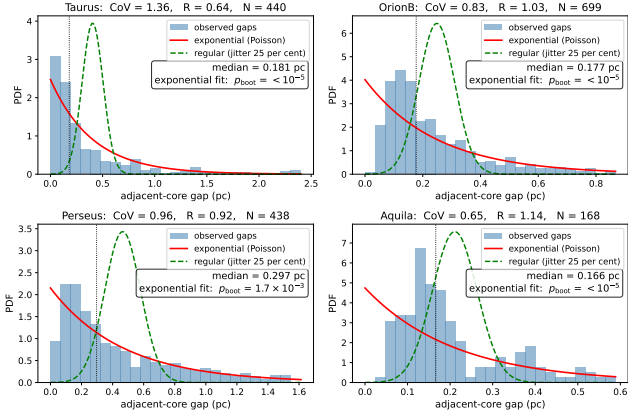
Adjacent-core gap distributions; p from parametric bootstrap with N_{\text{boot}} = 10^5
