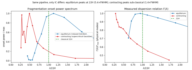
Figure 16. Equilibrium-recovery control (the primary validation that the sub-classical spectrum is not generated by the wavelength-extraction pipeline and is associated with the non-equilibrium initial state). The identical growth-rate measurement pipeline is applied to a relaxed, force-balanced pressure-confined Ostriker equilibrium (blue; prepared by explicit drag relaxation, then evolved drag-free) and to a dynamically contracting supercritical filament (orange); the two differ in their prepared initial state, not in the measurement, isolating the effect of starting from equilibrium versus contraction. Left : onset fragmentation power spectrum; the equilibrium peaks at the classical \lambda_m \approx 22H ( \approx 5.4 W_{\text{FWHM}} ) whereas the contracting filament places its shortest converged scale at \lesssim 1.4 W_{\text{FWHM}} , without a resolved maximum. Right : the dispersion relation \Gamma(\lambda) versus \lambda/22H ; the equilibrium shows the classical peak-and-decline with its maximum at 22H , whereas the contracting filament’s \Gamma rises monotonically. The pipeline thus recovers the classical wavelength when the physics is classical.
