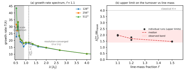
Figure 3. (a) Growth-rate spectrum \Gamma(\lambda) for a near-critical filament ( f = 1.1 ) at three resolutions. For \lambda \gtrsim 1\lambda_J the curves overlap; at the grid scale (shaded) they separate and rise with resolution. \Gamma plateaus rather than turning over, so \lambda_{\text{turn}}^{\text{lim}} \lesssim 1\lambda_J is an upper bound . (b) \lambda_{\text{turn}}^{\text{lim}}/W_{\text{FWHM}} against line-mass fraction, where W_{\text{FWHM}} is the FWHM of the evolved, projected simulation profile and not the initial half-width W_{\text{core}} or the beam-convolved observational W_{\text{fil}} (Table 5). The matched, beam-convolved Plummer bound is S_{\text{sim}}^{\text{upper}} \lesssim 1.0\text{--}1.3 (grey band; the \eta_W conversion is uncertain over 0.59–0.78, widening it by about a quarter).
