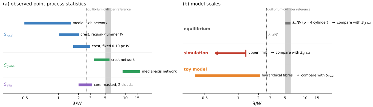
Figure 8. Observed statistics and model scales, kept apart. (a) The point-process quantities measured here: S_{\text{local}} under three structural and width conventions, S_{\text{global}} under two skeleton definitions, and the exploratory S_{\text{elig}} . Each bar spans the range across the four clouds. (b) Scales predicted by models, with the observable each would predict indicated: a one-bead-per-wavelength calculation predicts a line density and so should be set against S_{\text{global}} , whereas the hierarchical-fibre construction predicts the within-group separation and is closer to S_{\text{local}} . Neither correspondence is exact: S_{\text{global}} is the closest available proxy for a line density only if the measured length is fragmentation-eligible and velocity-coherent, which is not established here. The simulated entry is an upper limit and is drawn as an arrow. The grey band is the equilibrium-cylinder reference \lambda_m/W_{\text{FWHM}} \approx 5\text{--}6 for the projected p = 4 profile, exact for that equilibrium and not invariant for the observed p \simeq 2 profiles; the dotted line is \lambda_{\text{cr}} . No quantitative identification between a quantity in (a) and one in (b) is intended: they are shown on a common dimensionless axis only to compare magnitudes. The horizontal axis is symmetric-log below \lambda/W = 1 .
