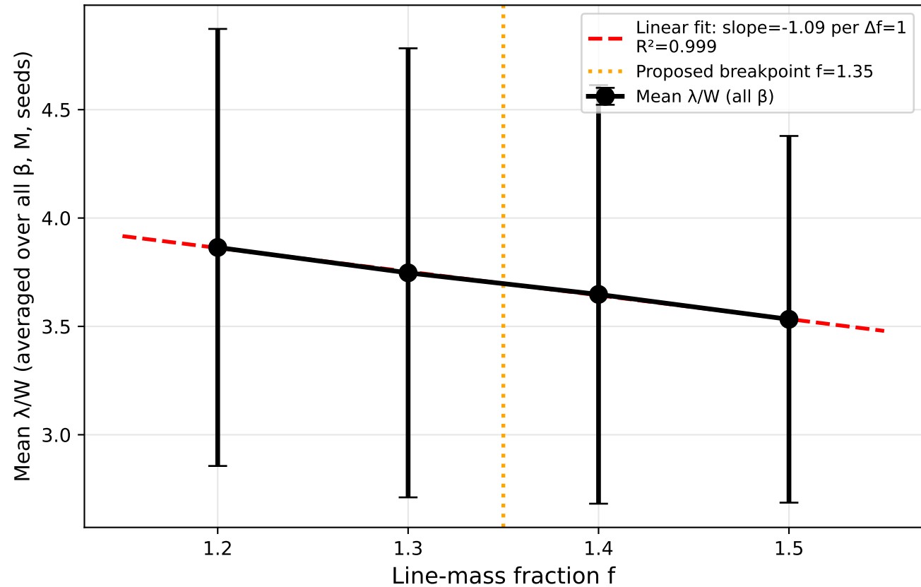
CTZM: Smooth vs discontinuous \lambda/W(f) Marginal mean — no discontinuity detected
