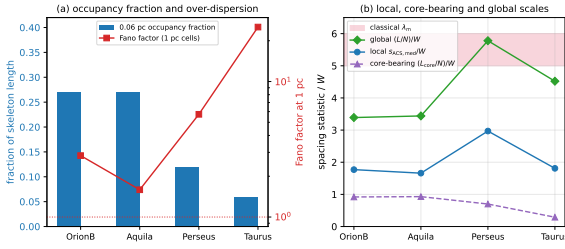
Figure 3. Spatial inhomogeneity of core occurrence along the filaments. (a) The 0.06 pc occupancy fraction (bars, left axis) is 6–27 per cent, while the Fano factor of counts in 1 pc cells (red, right axis, logarithmic) exceeds the Poisson value of unity in every cloud. (b) The three normalised spacing statistics: the local adjacent-core spacing is well below the reference band, the global (L/N)/W approaches it, and the core-bearing (L_{\text{core}}/N)/W lies below both because the occupied stretches are densely populated. The separation between the blue and green curves measures how unevenly the cores occupy the crest.
