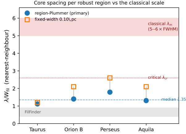
Figure 4. Nearest-neighbour core spacing per primary region ( s_{\text{med}}/W_{\text{fil}} ; Section 2.9), in the two DisPerSE width conventions: directly-measured region-Plummer widths (blue circles, preferred; per-region raw 1.1, 1.4, 1.8, 1.3, median 1.4, dashed) and the fixed 0.10 pc width (orange squares; 1.2, 2.1, 2.6, 2.1), both shown raw (before the injection–recovery correction; Section 2.7). The red band is the classical fastest-growing wavelength \lambda_m \approx 5\text{--}6 \times \text{FWHM} (Fischera & Martin 2012; = 4 \times the flat diameter, Inutsuka & Miyama 1992) and the dotted line the classical critical wavelength \lambda_{\text{cr}} \approx 2.6 \times \text{FWHM} ; every region lies well below both. The grey band marks the independent FilFinder skeleton range ( \lambda/W \approx 0.4\text{--}0.8 ). (Point ranges are descriptive, not confidence intervals; Section 2.10.)
