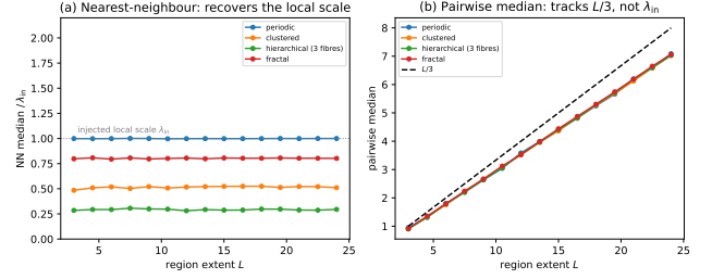
Figure 3. Synthetic validation that the nearest-neighbour (NN) statistic recovers the injected local spacing scale while the pairwise median does not (a clustered process need not possess a fragmentation wavelength). Cores are placed on a segment of extent L by four point processes (periodic, clustered, hierarchical three-fibre, fractal), each with a fixed injected local scale \lambda_{\text{in}} . (a) The NN median (normalised by \lambda_{\text{in}} ) is flat with L and recovers each process’s local/apparent scale (the hierarchical case gives \lambda_{\text{in}}/3 , the projected value). (b) The pairwise median instead rises along 0.293 L (dashed; this is the median of the triangular pairwise-distance law, whose mean is L/3 ; Appendix A) for all four processes, independent of \lambda_{\text{in}} — confirming that it measures the segment extent, not the fragmentation wavelength.
