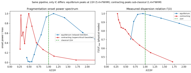
Figure 13. Equilibrium-recovery control (the primary validation that the sub-classical spectrum is not generated by the wavelength-extraction pipeline and is associated with the non-equilibrium initial state). The identical growth-rate measurement pipeline is applied to a relaxed, force-balanced pressure-confined Ostriker equilibrium (blue; prepared by explicit drag relaxation, then evolved drag-free) and to a dynamically contracting supercritical filament (orange); the two differ in their prepared initial state, not in the measurement, isolating the effect of starting from equilibrium versus contraction. Left : onset fragmentation power spectrum; the equilibrium peaks at the classical \lambda_m \approx 22H ( \approx 5.4 W_{\text{FWHM}} ) while the contracting filament peaks sub-classically ( \approx 1.4 W_{\text{FWHM}} , upper limit). Right : the dispersion relation \Gamma(\lambda) versus \lambda/22H ; the equilibrium shows the classical peak-and-decline with its maximum at 22H , whereas the contracting filament's \Gamma rises monotonically. The pipeline thus recovers the classical wavelength when the physics is classical.
