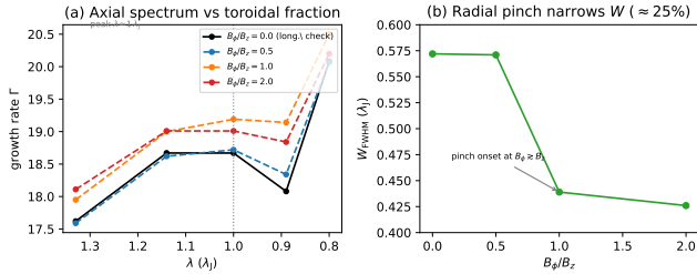
Figure 10. Divergence-free helical-field scan ( B_\phi/B_z = 0 – 2 , 512 \times 128^2 ; Section 4.3). (a) The axial growth-rate spectrum \Gamma(\lambda) in the physical band is invariant to the toroidal fraction ( < 6\% , fit noise), with the plateau peak fixed at \lambda \approx 1 \lambda_J ; B_\phi/B_z = 0 (black) reproduces the pure-longitudinal spectrum, a code check. No excess growth appears at shorter \lambda for any winding. (b) The one systematic effect is a radial pinch : the formation FWHM narrows by \approx 25\% , with onset at B_\phi \gtrsim B_z . The seeded helical field therefore raises \lambda/W by shrinking W , not by shortening \lambda ; the force-balanced Fiege & Pudritz (2000) pinch mode is not tested here.
