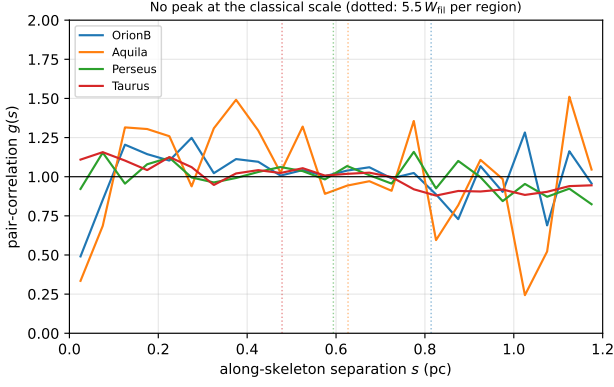
Figure 8. Along-skeleton pair-correlation function g(s) for the four primary clouds (uniform-random expectation on the matched components divided out; g = 1 is no correlation). Dotted vertical lines mark the classical scale 5.5 W_{\text{fil}} per region. No cloud shows a peak at the classical scale ( g \approx 1 there, slightly below unity in Orion B and Aquila); the only departures are a mild small-separation excess (Taurus) and weak region-envelope features near 1 pc. The classical periodic comb is therefore absent, consistent with a non-periodic, intermittent distribution bearing a small-scale exclusion (Section 2.11).
