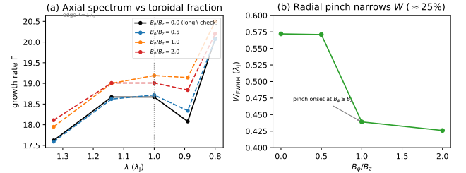
Figure 13. Divergence-free helical-field scan ( B_\phi/B_z = 0\text{--}2 , 512 \times 128^2 ; Section 4.3). (a) The axial growth-rate spectrum \Gamma(\lambda) in the physical band is invariant to the toroidal fraction ( < 6\% , fit noise), with the converged-band edge fixed at \lambda \approx 1 \lambda_J ; B_\phi/B_z = 0 (black) reproduces the pure-longitudinal spectrum, a code check. No excess growth appears at shorter \lambda for any winding. (b) The one systematic effect is a radial pinch : the formation FWHM narrows by \approx 25\% , with onset at B_\phi \gtrsim B_z . The seeded helical field therefore raises \lambda/W by shrinking W , not by shortening \lambda ; the force-balanced Fiege & Pudritz (2000) pinch mode is not tested here.
