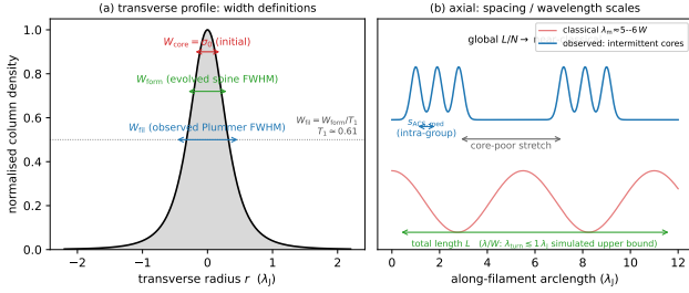
Figure 11. Schematic of the length-scale definitions used throughout (Table 1). (a) Transverse column-density profile, marking the initial half-width W_{\text{core}} = \sigma_0 , the evolved spine FWHM W_{\text{form}} , and the observed beam-convolved Plummer FWHM W_{\text{fil}} = W_{\text{form}}/T_1 ( T_1 \simeq 0.61 ; Eq. 6). (b) Axial view contrasting the classical widely-spaced comb ( \lambda_m \approx 5\text{--}6W ) with the observed intermittent cores: a short intra-group adjacent spacing s_{\text{ACS,med}} within core-rich stretches separated by core-poor filament, whose filament-averaged line density L/N is near-classical, while the simulated fragmentation scale is an upper bound \lambda_{\text{turn}} \lesssim 1 \lambda_J .
