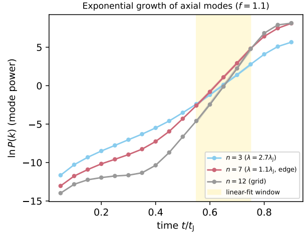
Figure 14. Power in three axial modes versus time for a near-critical filament ( f = 1.1 ). Each grows with an approximately exponential interval (the fit window, shaded) whose slope gives the growth rate; the growth steepens as the filament collapses, so the extracted rate characterises a dynamically collapsing filament. The representative mode at the converged-band edge, n = 7 , grows faster than the long-wavelength n = 3 , giving the sub-classical \lambda_{\text{turn}} ; the grid-scale n = 12 is shown for reference.
