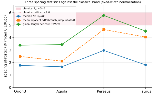
Figure 7. Three spacing statistics per cloud (single re-implementation, all normalised by the fixed 0.10 pc width so they are directly comparable), against the classical band (5–6, red; critical \approx 2.6 , dotted). The median along-skeleton ACS spacing (blue, \approx 1.7 –3.0) is sub-classical everywhere; the global length per core (L/N)/W (green, \approx 3.4 –5.8) is classical in Perseus, near-classical in Taurus, and sub-classical in Orion B and Aquila; the mean adjacent spacing (orange) lies between but is inflated by arclength branch-jumps. The factor \approx 2 gap between the blue and green points reflects the generic mean/median skew plus dilution by core-poor filament (a coverage effect), not small-scale clustering (Section 2.8): short adjacent spacing within core-bearing stretches, diluted by extensive core-free filament.
