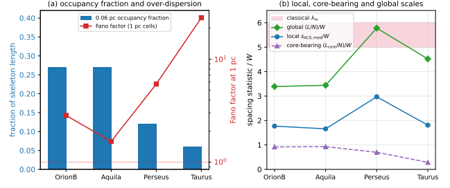
Figure 6. Intermittency of core formation along the filaments. (a) The 0.06 pc occupancy fraction (bars, left axis) is 6–27 per cent, while the Fano factor of counts in 1 pc cells (red, right axis, logarithmic) exceeds the Poisson value of unity in every cloud. (b) The three normalised spacing statistics: the local adjacent-core spacing is well below the classical band, the global (L/N)/W approaches it, and the core-bearing (L_{\text{core}}/N)/W lies below both because the occupied stretches are densely populated. The separation between the blue and green curves is the intermittency.
