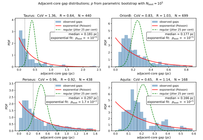
Figure 9. Adjacent-core gap distributions along the skeletons of the four primary regions (histograms), with exponential/Poisson (solid) and regular/periodic (dashed) reference curves; each panel gives the coefficient of variation CoV, the 1-D Clark–Evans ratio R , and the exponential goodness-of-fit p -value calibrated by parametric bootstrap ( p_{\text{boot}} ; the null distribution of the KS statistic is built by resampling from the fitted exponential, removing the estimated-parameter bias of the standard test). The result is two-sided: the regular/periodic model is rejected overwhelmingly ( p_{\text{boot}} < 10^{-5} , the parametric-bootstrap floor, 1/N_{\text{boot}} with N_{\text{boot}} = 10^5 ) in every region, and the pure-exponential (Poisson) model is also rejected ( p_{\text{boot}} < 10^{-5} (Perseus 1.7 \times 10^{-3} ) in all four), so the cores are neither periodic nor pure-Poisson; consistent with a point process that is locally exclusion-limited but over-dispersed on parsec scales (the deficit of small gaps, R > 1 ; largely instrumental).
