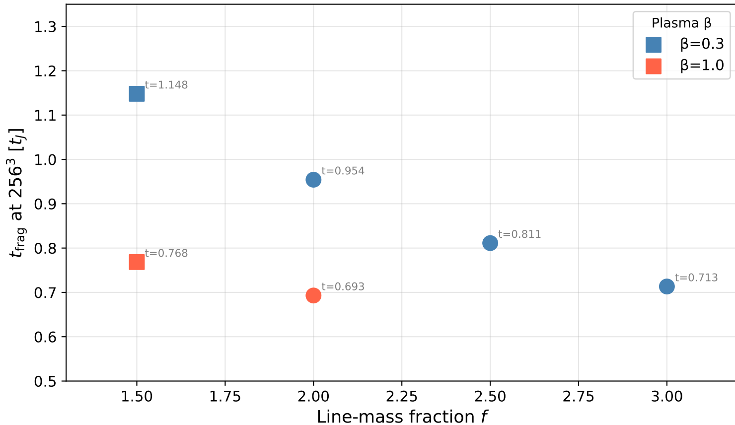
Priority 2: Resolution Convergence — 256^3 Fragmentation Times
