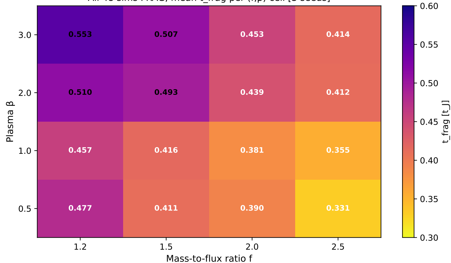
Campaign 1: Perpendicular B ( \theta=90^\circ ) — t_{\text{frag}} Heat Map All 48 sims FRAG, mean t_{\text{frag}} per (f, \beta ) cell [3 seeds]
