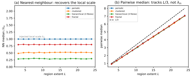
Figure 3. Synthetic validation that the nearest-neighbour (NN) statistic estimates the fragmentation scale while the pairwise median does not. Cores are placed on a segment of extent L by four point processes (periodic, clustered, hierarchical three-fibre, fractal), each with a fixed injected local scale \lambda_{in} . (a) The NN median (normalised by \lambda_{in} ) is flat with L and recovers each process’s local/apparent scale (the hierarchical case gives \lambda_{in}/3 , the projected value). (b) The pairwise median instead rises along 0.293 L (dashed; this is the median of the triangular pairwise-distance law, whose mean is L/3 ; Appendix A) for all four processes, independent of \lambda_{in} — confirming that it measures the region extent, not the fragmentation wavelength.
