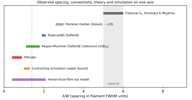
Figure 6. The full methodological envelope of \lambda/W on a single axis, showing that several distinct physical interpretations occupy the allowed observational region while all lie well below the classical value. Marked, from top: the classical band (5–6; Inutsuka & Miyama 1992; Fischera & Martin 2012); the biased pairwise median ( \approx L/3 ); fixed-width DisPerSE (1.9–2.1); region-Plummer DisPerSE (our reference NN-spacing ratio (\lambda/W)_0 \approx 1.4 ); FilFinder (0.4–0.9 across correction states; raw 0.5–0.9, Table 3); the contracting-simulation upper bound (1.0–1.3); and the hierarchical-fibre toy-model range. Because the observational conventions, the simulated upper bound and the fibre toy model all overlap well below the classical band, the sub-classical sign is robust while its magnitude is convention-dominated (Section 2.12); the comparison with simulation (Section 5) should be read against this envelope, not against a single number.
