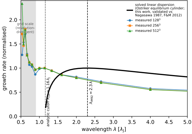
Figure B2. The from-scratch-solved eigenvalue dispersion relation of the isothermal equilibrium cylinder (Nagasawa 1987; Inutsuka & Miyama 1992), validated to < 1% against Nagasawa (1987) and Fischera & Martin (2012) (not a fit): it peaks at \lambda_{\text{IM92}} \approx 2.3 \lambda_J and vanishes at the cutoff \lambda_{\text{cr}} \approx 1.2 \lambda_J , overplotted on the measured growth-rate spectrum ( f = 1.1 , three resolutions, normalised at \lambda = 1.14 \lambda_J ). The measured spectrum instead rises monotonically into the grid-scale region (shaded), confirming the small-scale rise is numerical. The measured wavelength ( \approx 1.1 \lambda_J ; \lambda_{\text{max}}/W_{\text{FWHM}} \approx 2 ) lies a factor \approx 2.5 –3 below the analytic peak ( 5 – 6 \times \text{FWHM} ) and near the cutoff, so we treat it as an order- \lambda_J , sub-classical value, not a precisely-located maximum.
