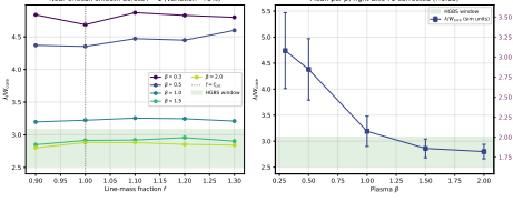
Figure E3. Near-critical runs: \lambda/W_{\text{core}} across f = 0.9 – 1.3 for five \beta values, smooth with no discontinuity at f = 1.0 (left); mean per \beta (right). The convergence-independent quantity is \lambda/W_{\text{core}} ; the observable follows from \lambda/W_{\text{fil}} \approx 0.27 (\lambda/W_{\text{core}}) (Eq. 6), so the highest- \beta points correspond to \lambda/W_{\text{fil}} \approx 0.75 – 0.8 . This near-critical calibration lies below the observed spacing under any convention (Table 3); the primary simulated value is the growth-rate wavelength (an upper limit; Section 5), not this ratio.
