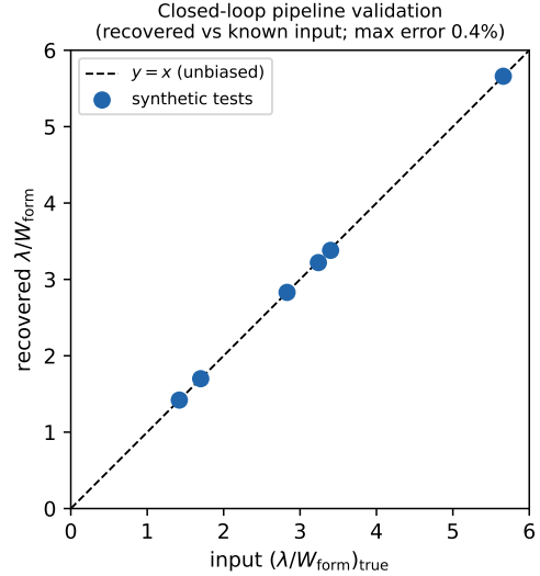
Figure B1. Closed-loop validation: the pipeline recovers the injected \lambda/W to within 0.4% over \lambda/W = 1.4 – 5.7 .
