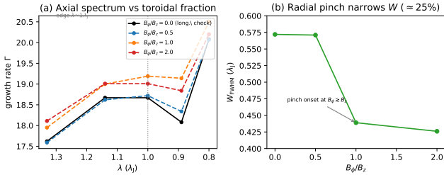
Figure 14. Divergence-free helical-field scan ( B_\phi/B_z = 0 – 2 , 512 \times 128^2 ; Section 4.3). (a) The axial growth-rate spectrum \Gamma(\lambda) in the physical band is invariant to the toroidal fraction ( < 6\% , fit noise), with the converged-band edge fixed at \lambda \approx 1 \lambda_J ; B_\phi/B_z = 0 (black) reproduces the pure-longitudinal spectrum, a code check. No excess growth appears at shorter \lambda for any winding. (b) The one systematic effect is a radial pinch : the formation FWHM narrows by \approx 25\% , with onset at B_\phi \gtrsim B_z . The seeded helical field therefore raises \lambda/W by shrinking W , not by shortening \lambda ; the force-balanced Fiege & Pudritz (2000) pinch mode is not tested here.
