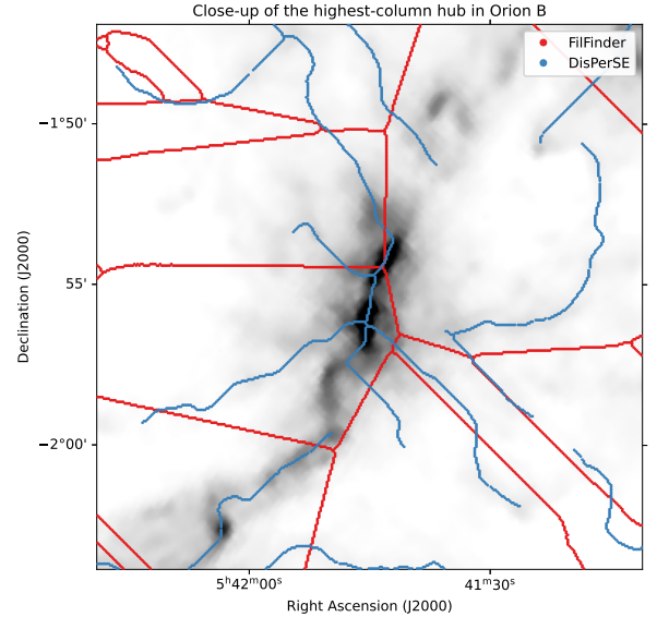
Figure 6. Close-up of the highest-column hub in Orion B, showing where the two algorithms actually differ. DisPerSE (blue) tracks the visible crests. FilFinder (red) reproduces the main ridge but adds long, nearly straight spokes that radiate from the hub and do not follow the greyscale emission: these are medial-axis artefacts of a large connected mask rather than resolved sub-filaments. The extra FilFinder length is therefore not obviously tracing real hierarchical structure, which is why we carry the FilFinder branch as the extreme of the convention envelope rather than as an equally-weighted alternative.
