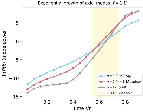
Figure 15. Power in three axial modes versus time for a near-critical filament ( f = 1.1 ). Each grows with an approximately exponential interval (the fit window, shaded) whose slope gives the growth rate; the growth steepens as the filament collapses, so the extracted rate characterises a dynamically collapsing filament. The representative mode at the converged-band edge, n = 7 , grows faster than the long-wavelength n = 3 , giving the sub-classical \lambda_{\text{turn}} ; the grid-scale n = 12 is shown for reference.
