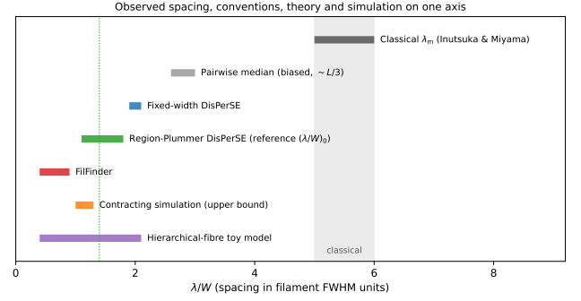
Figure 11. The full methodological envelope of \lambda/W on a single axis, showing that several distinct physical interpretations occupy the allowed observational region while all lie well below the classical value. Marked, from top: the classical band (5–6; Inutsuka & Miyama 1992; Fischera & Martin 2012); the biased pairwise median ( \approx L/3 ); fixed-width DisPerSE (1.9–2.1); region-Plummer DisPerSE (our reference ACS-spacing ratio (s_{\text{ACS,med}}/W)_0 \approx 1.4 ); FilFinder (0.4–0.8, Table 3); the contracting-simulation upper bound (1.0–1.3); and the hierarchical-fibre toy-model range. Because the observational conventions, the simulated upper bound and the fibre toy model all overlap well below the classical band, the sub-classical sign is robust while its magnitude is convention-dominated (Section 2.16); the comparison with simulation (Section 5) should be read against this envelope, not against a single number.
