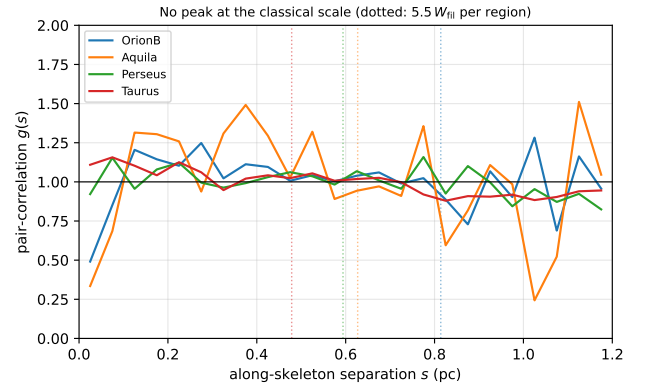
Figure 9. Along-skeleton pair-correlation function g(s) for the four primary clouds (uniform-random expectation on the matched components divided out; g = 1 is no correlation). Dotted vertical lines mark the classical scale 5.5 W_{\text{fil}} per region. No cloud shows a peak at the classical scale ( g \approx 1 there, slightly below unity in Orion B and Aquila); the only departures are a mild small-separation excess (Taurus) and weak region-envelope features near 1 pc. The classical periodic comb is therefore absent, consistent with a non-periodic, intermittent distribution bearing a small-scale exclusion (Section 2.12).
