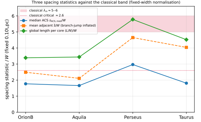
Figure 8. Three spacing statistics per cloud (single re-implementation, all normalised by the fixed 0.10 pc width so they are directly comparable), against the classical band (5–6, red; critical \approx 2.6 , dotted). The median along-skeleton ACS spacing (blue, \approx 1.7 – 3.0 ) is sub-classical everywhere; the global length per core (L/N)/W (green, \approx 3.4 – 5.8 ) is classical in Perseus, near-classical in Taurus, and sub-classical in Orion B and Aquila; the mean adjacent spacing (orange) lies between but is inflated by arclength branch-jumps. The factor- \approx 2 gap between the blue and green points reflects the generic mean/median skew plus dilution by core-poor filament (a coverage effect), not small-scale clustering (Section 2.8): short adjacent spacing within core-bearing stretches, diluted by extensive core-free filament.
