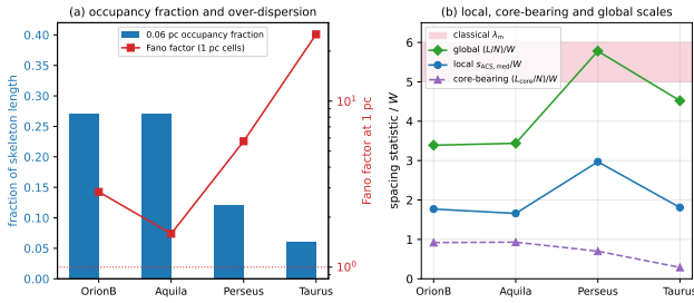
Figure 7. Intermittency of core formation along the filaments. (a) The 0.06 pc occupancy fraction (bars, left axis) is 6–27 per cent, while the Fano factor of counts in 1 pc cells (red, right axis, logarithmic) exceeds the Poisson value of unity in every cloud. (b) The three normalised spacing statistics: the local adjacent-core spacing is well below the classical band, the global (L/N)/W approaches it, and the core-bearing (L_{\text{core}}/N)/W lies below both because the occupied stretches are densely populated. The separation between the blue and green curves is the intermittency.
