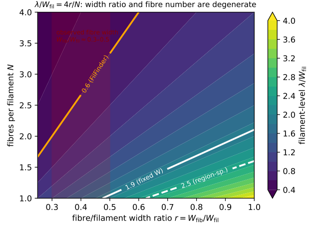
Figure 14. Hierarchical-fibre forward-model, showing the filament-level \lambda/W_{\text{fil}} recovered by our NN pipeline as a function of the fibre-to-filament width ratio r = W_{\text{fib}}/W_{\text{fil}} and the number of fibres N ; the model follows \lambda/W_{\text{fil}} \approx 4r/N (Eq. 12). White contours mark the observed fixed-width and region-specific values, the orange contour the FilFinder value, and the red band the observed fibre-width range ( r \approx 0.3\text{--}0.5 ). The observation constrains the combination r/N , not N alone: the sub-classical value is reproduced by a single narrow fibre, by a few wider fibres, or by intermediate combinations.
