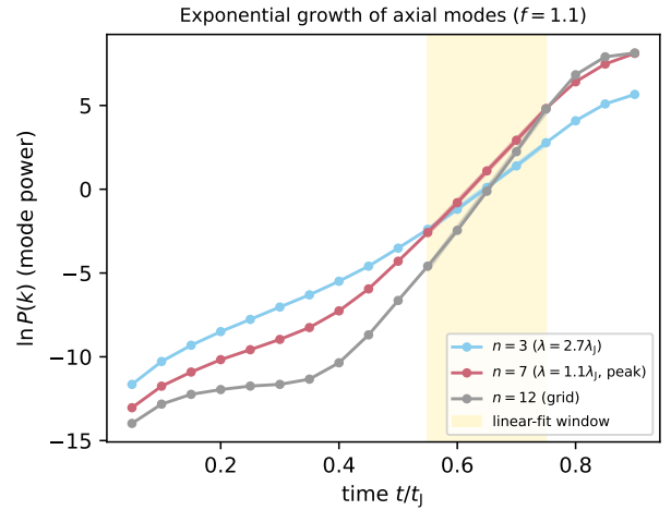
Figure 12. Power in three axial modes versus time for a near-critical filament ( f = 1.1 ). Each grows with an approximately exponential interval (the fit window, shaded) whose slope gives the growth rate; the growth steepens as the filament collapses, so the extracted rate characterises the dominant mode of a dynamically collapsing filament. The peak mode n=7 grows faster than the long-wavelength n=3 , giving the sub-classical \lambda_{\text{max}} ; the grid-scale n=12 is shown for reference.
