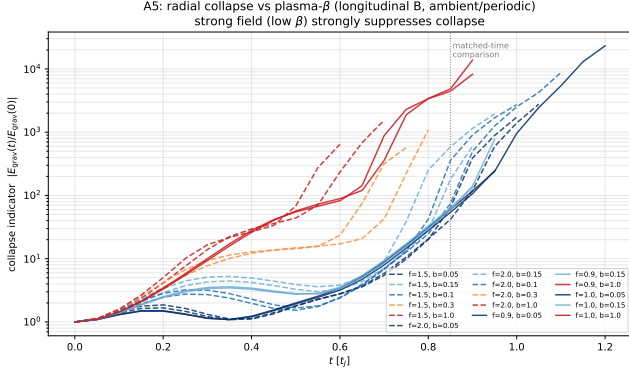
Figure 4. Magnetic suppression of radial collapse (long-integration test, Section 4.3). The collapse indicator |E_{\text{grav}}(t)/E_{\text{grav}}(0)| at matched time t = 0.85 t_J versus \beta , for f = 0.9 – 2.0 . Strong-field runs ( \beta \lesssim 0.15 ) remain at \sim 40 – 180 while weak-field runs ( \beta \gtrsim 0.3 – 1 ) run away to \sim 600 – 4600 : a clean \sim 1 – 2 dex magnetic suppression operating even for thermally supercritical filaments, the mechanism behind Fig. 5’s magnetically subcritical regime.
