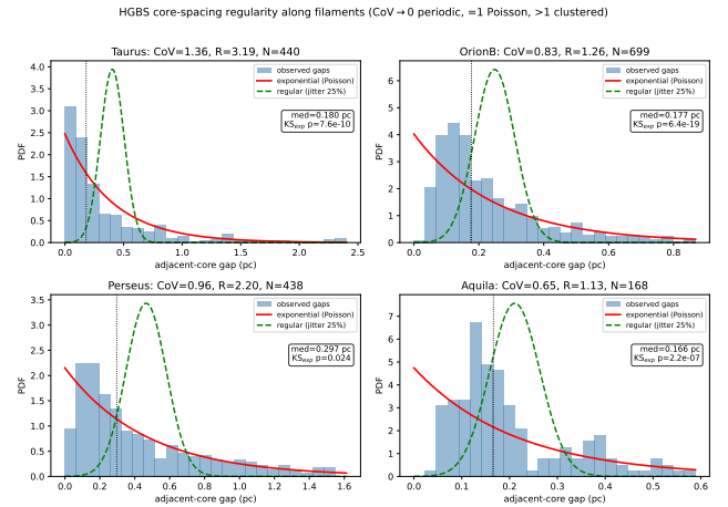
Figure 3. Adjacent-core gap distributions along the skeletons of the four robust regions (histograms), with exponential/Poisson (solid) and regular/periodic (dashed) reference curves; each panel is annotated with the coefficient of variation \text{CoV} and the 1-D Clark–Evans ratio R . \text{CoV} of order unity and the overwhelming rejection of the periodic model ( p \lesssim 10^{-15} ) show the cores are random-to-clustered, not periodically spaced.
