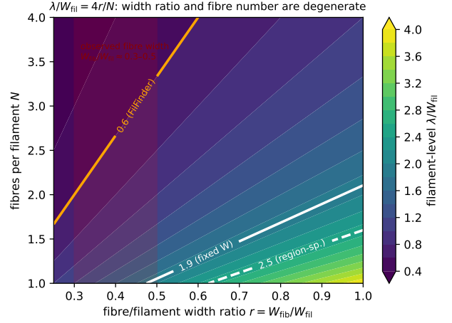
Figure 14. Hierarchical-fibre forward-model, showing the filament-level \lambda/W_{\text{fil}} recovered by our NN pipeline as a function of the fibre-to-filament width ratio r = W_{\text{fb}}/W_{\text{fil}} and the number of fibres N ; the model follows \lambda/W_{\text{fil}} \approx 4r/N (Eq. 12). White contours mark the observed fixed-width and region-specific values, the orange contour the FilFinder value, and the red band the observed fibre-width range ( r \approx 0.3 – 0.5 ). The observation constrains the combination r/N , not N alone: the sub-classical value is reproduced by a single narrow fibre, by a few wider fibres, or by intermediate combinations.
