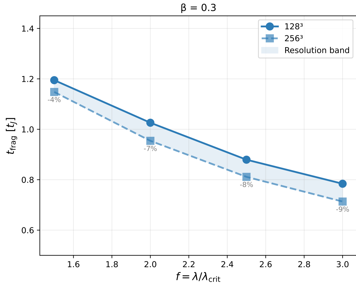
t_{\text{frag}} vs f : Resolution Dependence by \beta
