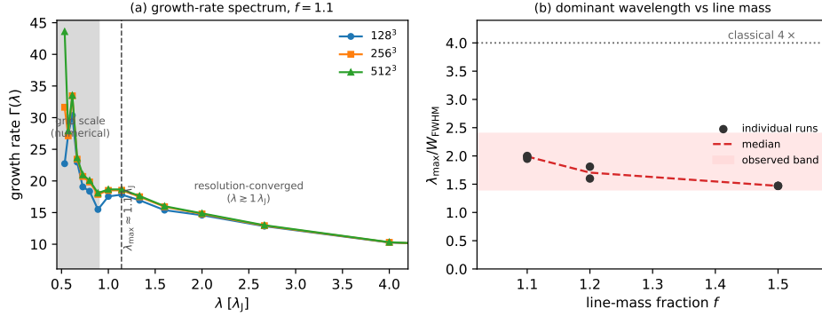
Figure 8. (a) Growth-rate spectrum \Gamma(\lambda) of the axial modes for a near-critical filament ( f = 1.1 ) at three resolutions. For \lambda \gtrsim 1 \lambda_J the curves overlap (resolution-converged); at the grid scale ( \lambda \lesssim 0.9 \lambda_J , shaded) they separate and rise with resolution, the signature of unresolved sub-fragmentation. The shaded grid-scale band corresponds to the axial cell size \Delta x = L_x/N (with L_x = 8 \lambda_J : \Delta x \approx 0.063, 0.031, 0.016 \lambda_J at 128^3, 256^3, 512^3 ). \Gamma plateaus (does not turn over) at the converged-band edge, so \lambda_{\max} \lesssim 1 \lambda_J is an upper bound , not a resolved maximum. (b) \lambda_{\max}/W_{\text{FWHM}} versus line-mass fraction (Gaussian FWHM), well below the classical 5–6 at every f . The like-for-like comparison uses a beam-convolved Plummer width \sim 1.5\times broader, giving matched \lambda/W \approx 1.0\text{--}1.3 (grey band): this, not the Gaussian \approx 2 , is what should be set against the observed \lambda/W \approx 0.4\text{--}1.9 .
