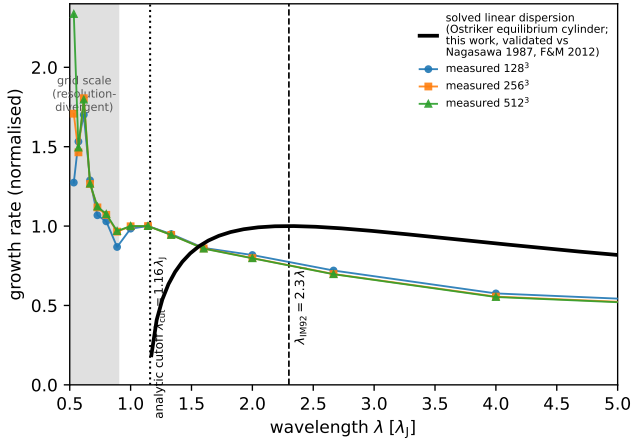
Figure B2. The from-scratch-solved eigenvalue dispersion relation of the isothermal equilibrium cylinder (Nagasawa 1987; Inutsuka & Miyama 1992), validated to < 1\% against Nagasawa (1987) and Fischera & Martin (2012) (not a fit): it peaks at \lambda_{IM92} \approx 2.3 \lambda_J and vanishes at the cutoff \lambda_{cr} \approx 1.2 \lambda_J , overplotted on the measured growth-rate spectrum ( f = 1.1 , three resolutions, normalised at \lambda = 1.14 \lambda_J ). The measured spectrum instead rises monotonically into the grid-scale region (shaded), confirming the small-scale rise is numerical. The measured wavelength ( \approx 1.1 \lambda_J ; \lambda_{max}/W_{FWHM} \approx 2 ) lies a factor \approx 2.5 – 3 below the analytic peak ( 5 – 6 \times FWHM ) and near the cutoff, so we treat it as an order- \lambda_J , sub-classical value, not a precisely-located maximum.
