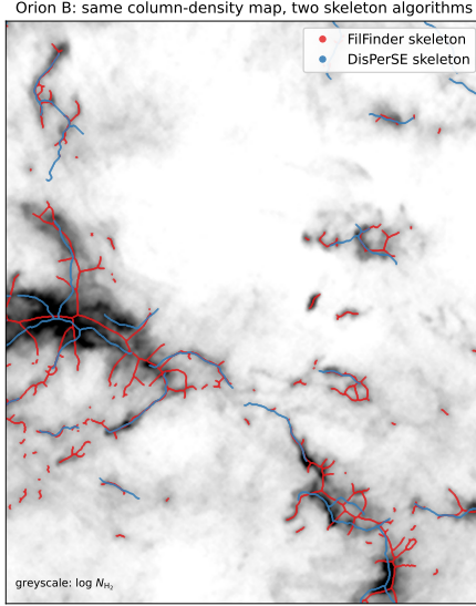
Figure 4. The dominant observational systematic, shown directly: the DisPerSE (blue) and FilFinder (red) skeletons extracted from the same Herschel column-density map of Orion B (greyscale, \log N_{\text{H}_2} ; a representative sub-region). The two algorithms trace substantially different filament networks — FilFinder’s medial axis of a column-density mask is denser and more branched and follows more low-contrast material, whereas DisPerSE follows the persistent crests — which is why the inferred \lambda/W differs by a factor of \sim 2 between them (Section 2.9). The difference is intrinsic to how each algorithm defines a “filament” and is not removed by tuning; it is the largest single uncertainty on the magnitude of the spacing, though the sub-classical sign holds for both.
