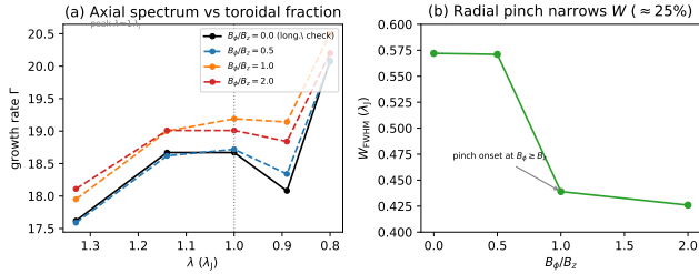
Figure 6. Divergence-free helical-field scan ( B_\phi/B_z = 0 – 2 , 512 \times 128^2 ; Section 4.3). (a) The axial growth-rate spectrum \Gamma(\lambda) in the physical band is invariant to the toroidal fraction ( < 6\% , fit noise), with the plateau peak fixed at \lambda \approx 1 \lambda_J ; B_\phi/B_z = 0 (black) reproduces the pure-longitudinal spectrum, a code check. No excess growth appears at shorter \lambda for any winding. (b) The one systematic effect is a radial pinch : the formation FWHM narrows by \approx 25\% , with onset at B_\phi \gtrsim B_z . The seeded helical field therefore raises \lambda/W by shrinking W , not by shortening \lambda ; the force-balanced Fiege & Pudritz (2000) pinch mode is not tested here.
