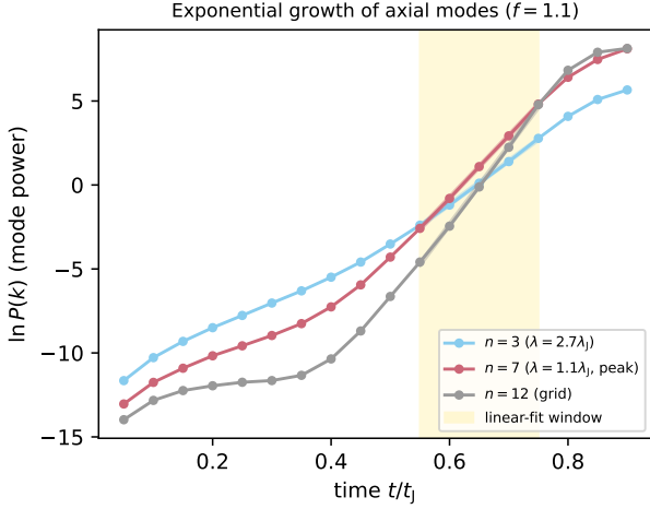
Figure 7. Power in three axial modes versus time for a near-critical filament ( f = 1.1 ). Each grows with an approximately exponential interval (the fit window, shaded) whose slope gives the growth rate; the growth steepens as the filament collapses, so the extracted rate characterises the dominant mode of a dynamically collapsing filament. The peak mode n = 7 grows faster than the long-wavelength n = 3 , giving the sub-classical \lambda_{\max} ; the grid-scale n = 12 is shown for reference.
