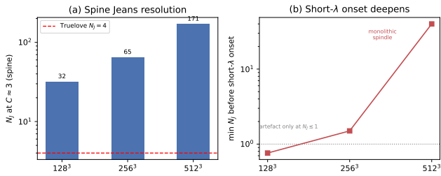
Figure 9. Ideal perpendicular-field refinement ladder ( 128^3-512^3 ; Section 4.6). (a) Cells per local Jeans length N_J at the beading-relevant spine contrast C \approx 3 : the collapsing spine is resolved far above the Truelove threshold ( N_J = 4 , dashed) at every resolution. (b) The spurious short- \lambda axial “beading” emerges only once the spine drops below N_J \approx 1 , and refinement pushes that onset to ever-deeper collapse (at 512^3 the filament stays monolithic to N_J \approx 40 at C \approx 30 ) — the signature of a grid artefact, not a physical fragmentation mode.
