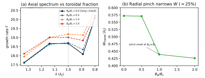
Figure 10. Divergence-free helical-field scan ( B_\phi/B_z = 0-2 , 512 \times 128^2 ; Section 4.6). (a) The axial growth-rate spectrum \Gamma(\lambda) in the physical band is invariant to the toroidal fraction ( < 6\% , fit noise), with the plateau peak fixed at \lambda \approx 1 \lambda_J ; B_\phi/B_z = 0 (black) reproduces the pure-longitudinal spectrum, a code check. No excess growth appears at shorter \lambda for any winding. (b) The one systematic effect is a radial pinch : the formation FWHM narrows by \approx 25\% , with onset at B_\phi \gtrsim B_z . The seeded helical field therefore raises \lambda/W by shrinking W , not by shortening \lambda ; the force-balanced Fiege & Pudritz (2000) pinch mode is not tested here.
