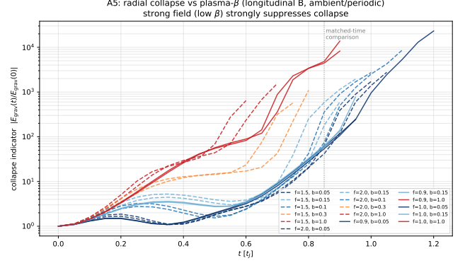
Figure 4. Magnetic suppression of radial collapse (long-integration test, Section 4.2). The collapse indicator |E_{\text{grav}}(t)/E_{\text{grav}}(0)| at matched time t = 0.85 t_J versus \beta , for f = 0.9 –2.0. Strong-field runs ( \beta \lesssim 0.15 ) remain at \sim 40 –180 while weak-field runs ( \beta \gtrsim 0.3 –1) run away to \sim 600 –4600: a clean \sim 1 –2 dex magnetic suppression operating even for thermally supercritical filaments, the mechanism behind Fig. D1’s magnetically supported (pressure-stabilised) regime.
