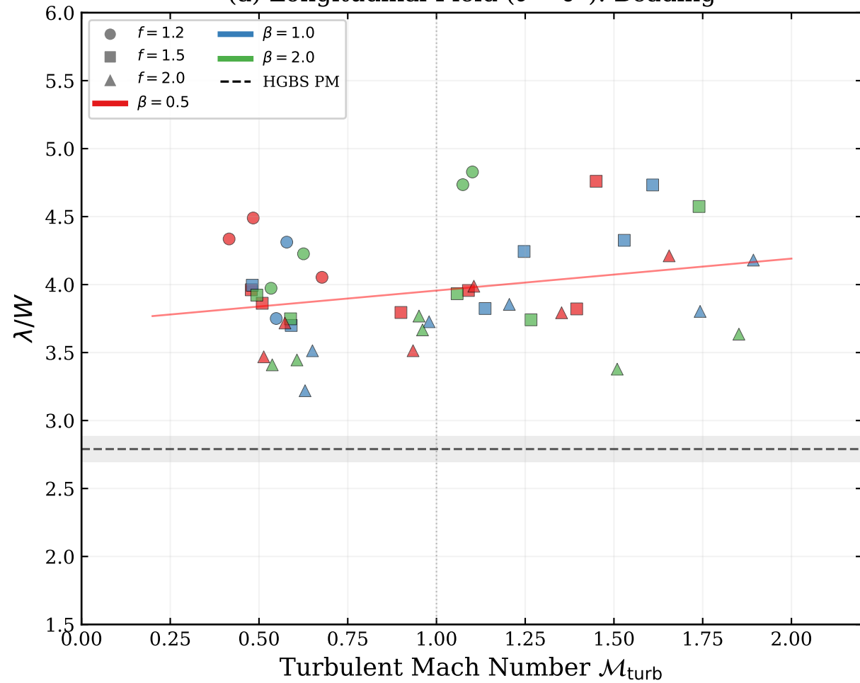
(a) Longitudinal Field ( \theta = 0^\circ ): Beading
