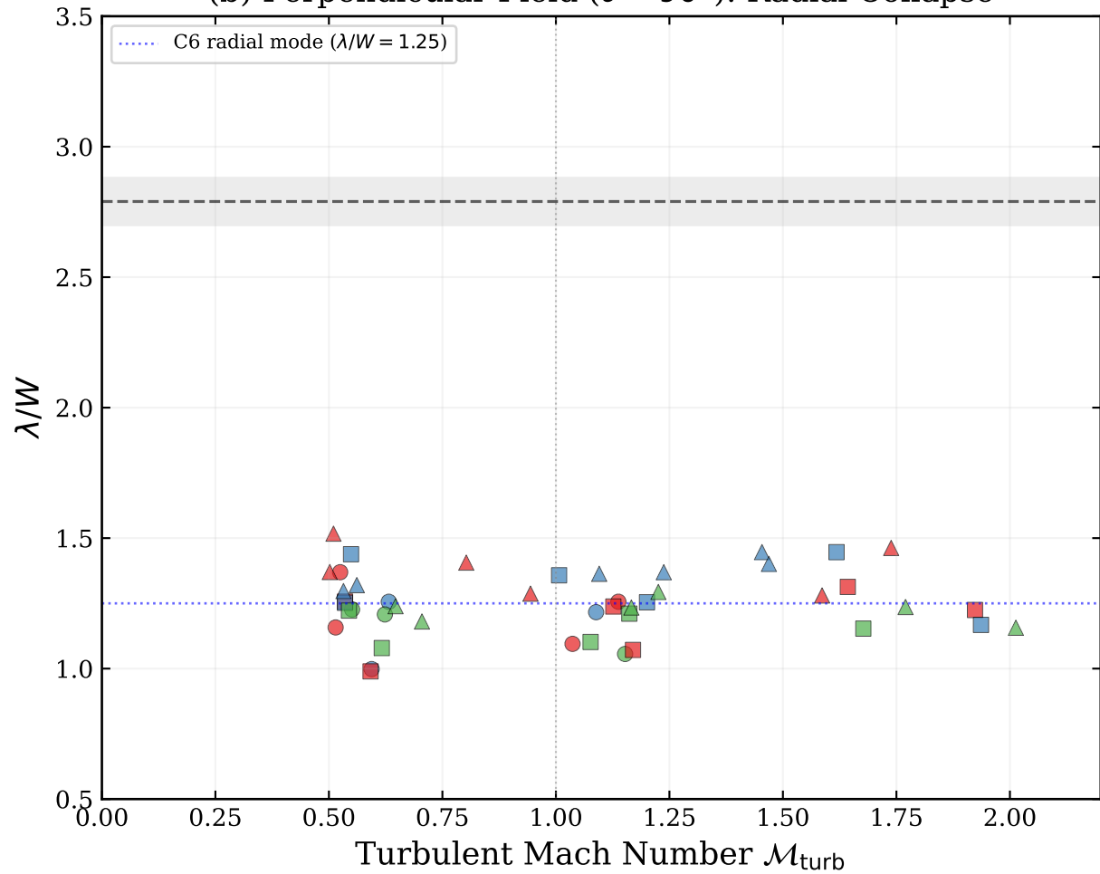
(b) Perpendicular Field ( \theta = 90^\circ ): Radial Collapse
