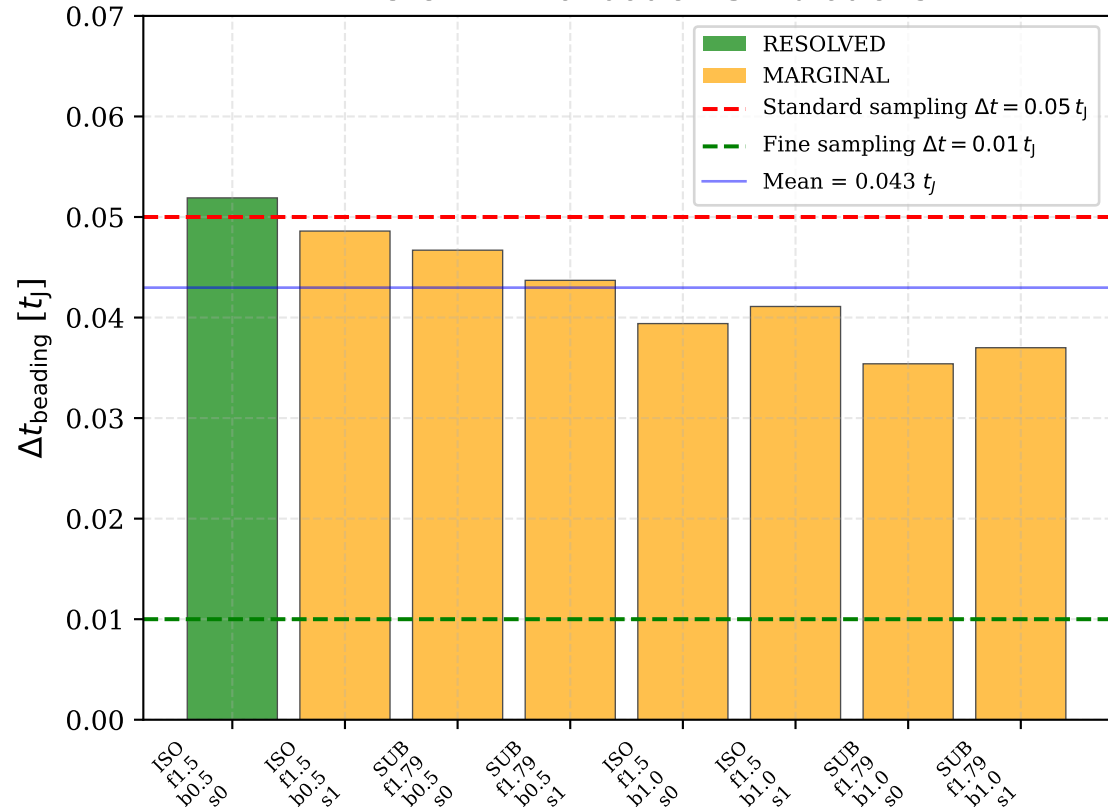
(b) Beading Detection Window Width All 8 CTZM Validation Simulations
