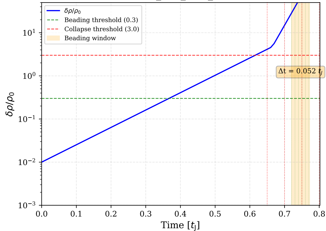
(a) Density Perturbation Growth (ISO_f1.5_b0.5_s0)
