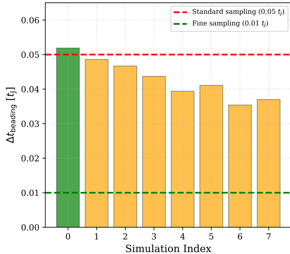
(a) CTZM: Beading Window (Referee #4)
