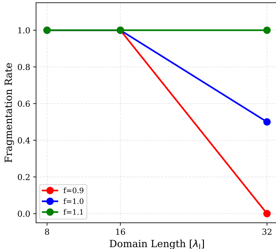
(b) Domain Convergence (Referee #7)
