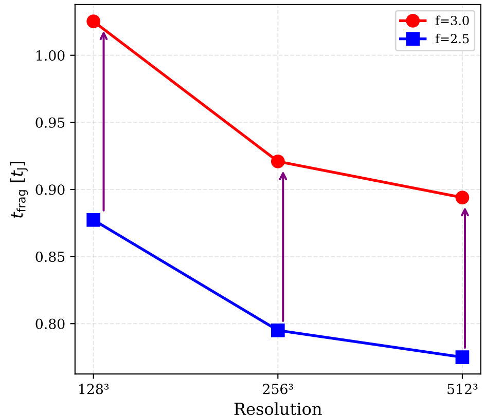
(c) Hourglass: Inverted f-dep. (Referee #10)
