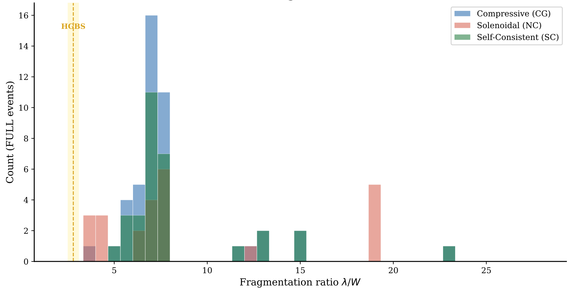
Distribution of \lambda/W — All Fragmentation Events (CG+NC+SC)
