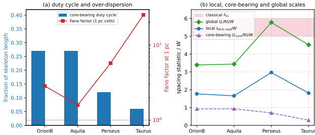
Figure 6. Intermittency of core formation along the filaments. (a) The core-bearing duty cycle (bars, left axis) is 6–27 per cent, while the Fano factor of counts in 1 pc cells (red, right axis, logarithmic) exceeds the Poisson value of unity in every cloud. (b) The three normalised spacing statistics: the local adjacent-core spacing is well below the classical band, the global (L/N)/W approaches it, and the core-bearing (L_{\text{core}}/N)/W lies below both because the occupied stretches are densely populated. The separation between the blue and green curves is the intermittency.
