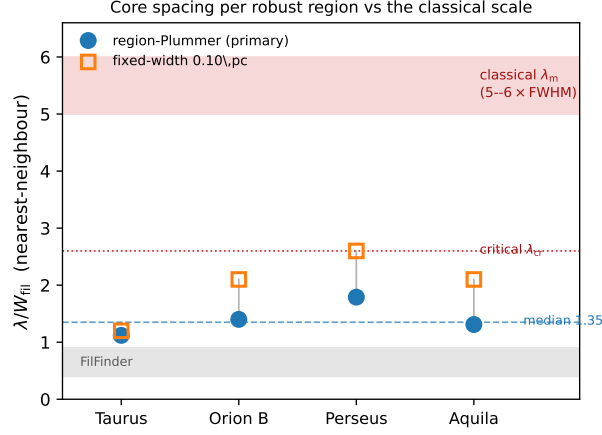
Figure 4. Adjacent-core (ACS) spacing per primary region ( s_{\text{ACS,med}}/W_{\text{fil}} ), the conditional descriptor measured within core-bearing stretches; the unconditional line density L/N , which is what fragmentation theory predicts, is shown in Fig. 6, in the two DisPerSE width conventions: directly-measured region-Plummer widths (blue circles, preferred; per-region raw 1.1, 1.4, 1.8, 1.3, dashed line at the median, which we quote as 1.4, the rounded value of the exact median of 1.35) and the fixed 0.10 pc width (orange squares; 1.2, 2.1, 2.6, 2.1), both shown raw (before the injection–recovery correction; Section 2.7). The red band is the classical fastest-growing wavelength \lambda_m \approx 5\text{--}6 \times \text{FWHM} (Fischera & Martin 2012; = 4 \times the flat diameter, Inutsuka & Miyama 1992) and the dotted line the classical critical wavelength \lambda_{\text{cr}} \approx 2.6 \times \text{FWHM} ; every region lies well below both. The grey band marks the independent FilFinder skeleton range ( \lambda/W \approx 0.4\text{--}0.8 ). (Uncertainty convention: Section 2.12.)
