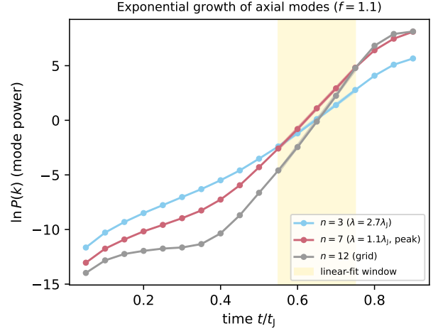
Figure 14. Power in three axial modes versus time for a near-critical filament ( f = 1.1 ). Each grows with an approximately exponential interval (the fit window, shaded) whose slope gives the growth rate; the growth steepens as the filament collapses, so the extracted rate characterises the dominant mode of a dynamically collapsing filament. The peak mode n = 7 grows faster than the long-wavelength n = 3 , giving the sub-classical \lambda_{\text{turn}} ; the grid-scale n = 12 is shown for reference.
