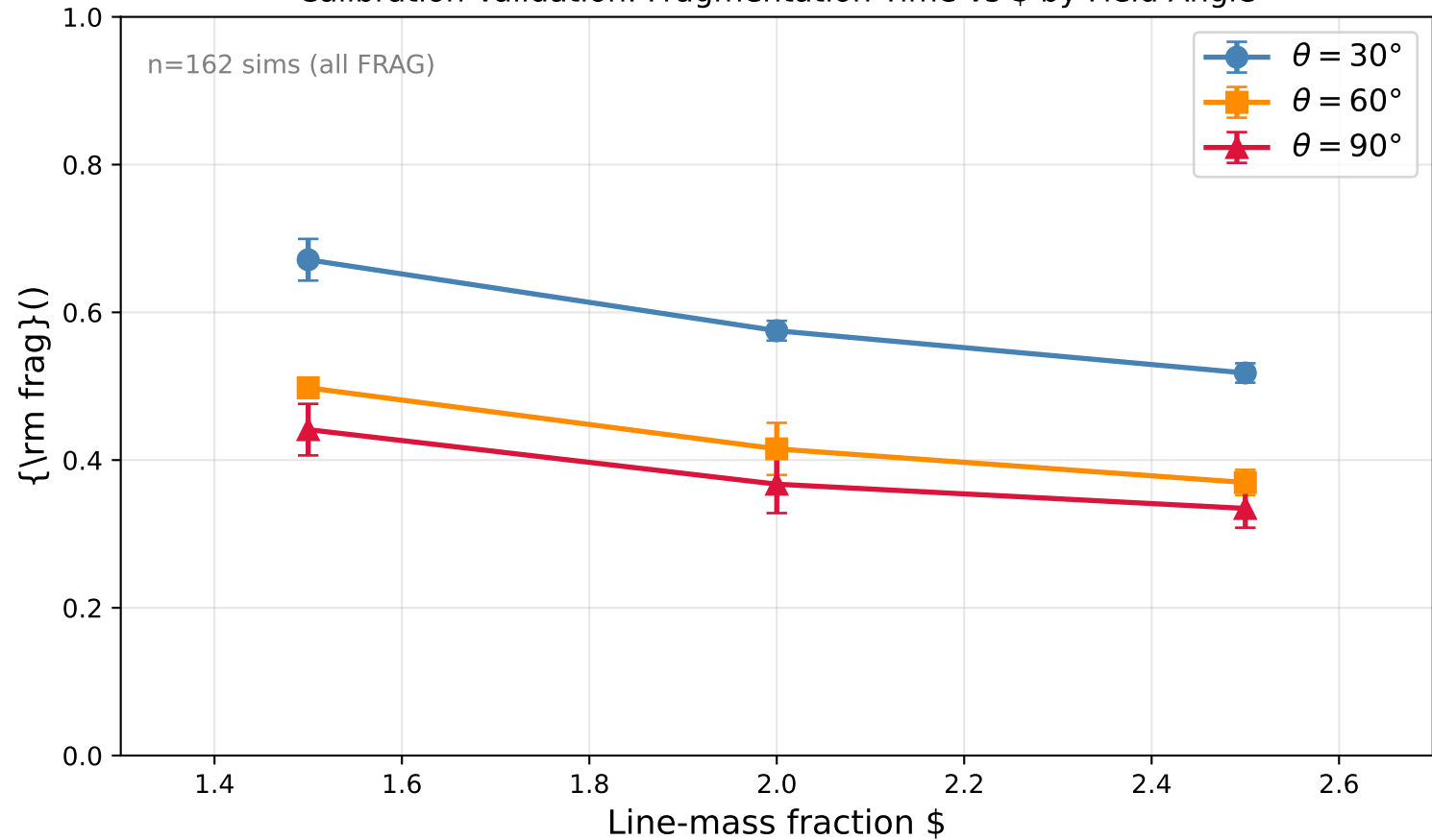
Calibration Validation: Fragmentation Time vs \xi by Field Angle
