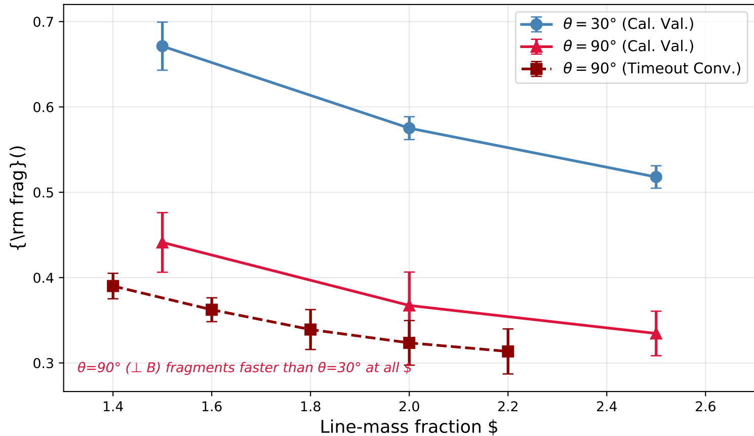
Effect of Field Angle on Fragmentation: \theta = 30^\circ vs \theta = 90^\circ
