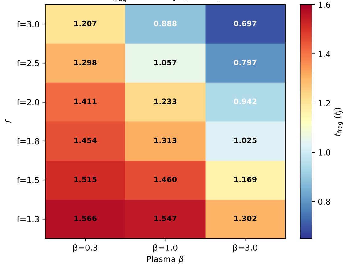
t_{\text{frag}} heatmap ( \theta = 0^\circ )
