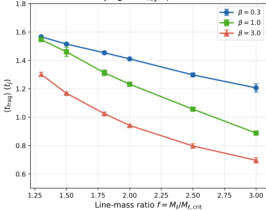
Campaign B: t_{\text{frag}}(f, \beta) at \theta = 0^\circ
