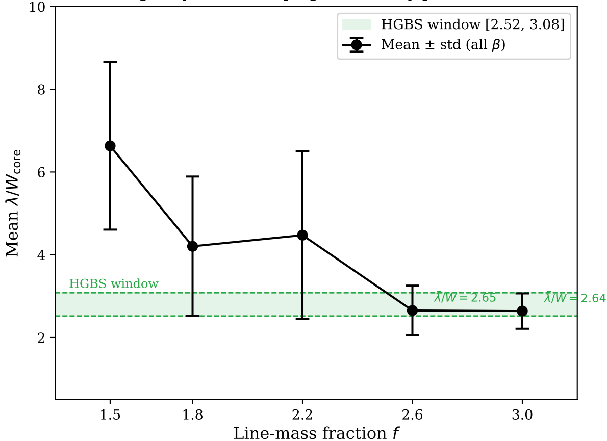
Rigid Cylinder Campaign: summary per f -value
