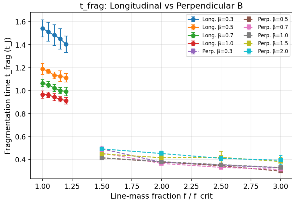
Fig 2: Field Geometry Effect on Fragmentation Timescale
