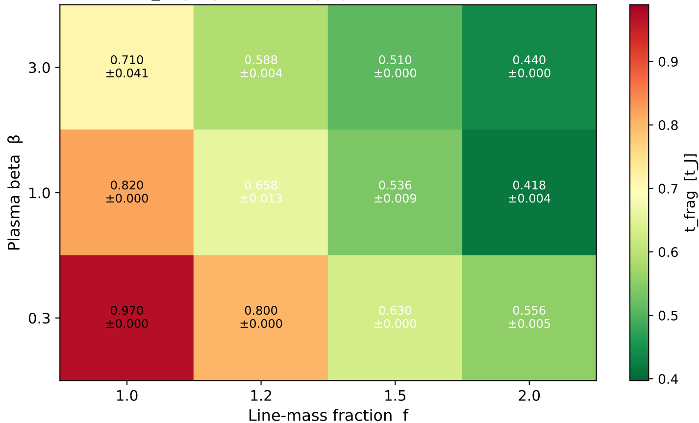
PFS: t_{\text{frag}}(f, \beta) [ \theta = 90^\circ , perpendicular B, 5 seeds/cell]
