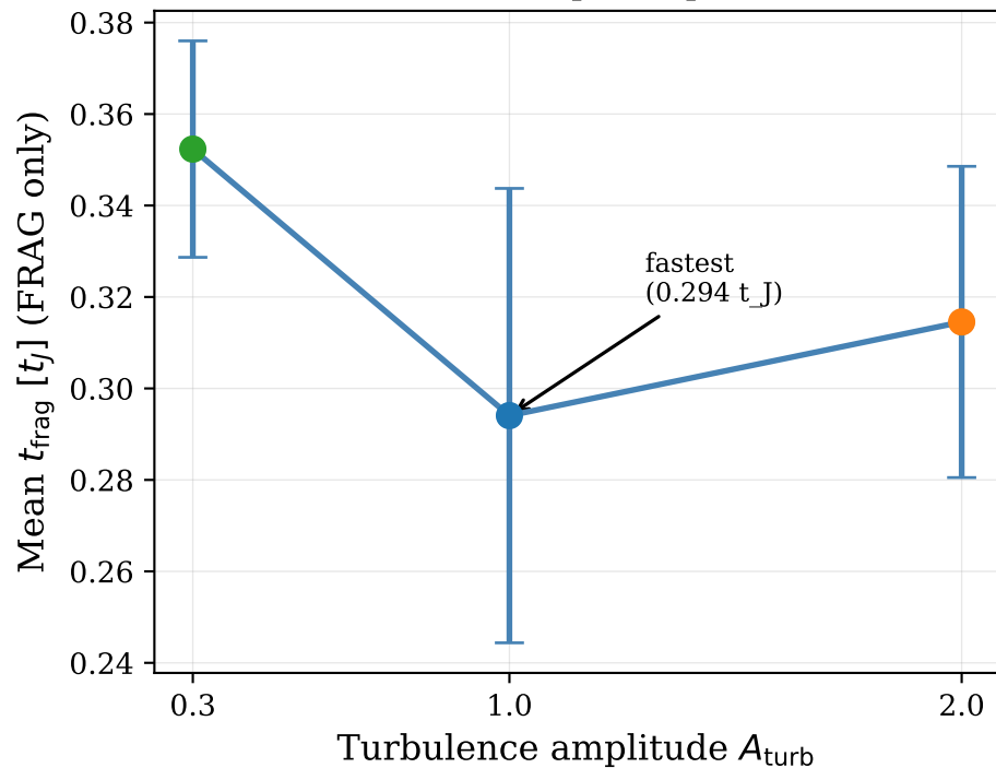
(b) Non-monotonic: peak speed at A=1.0
