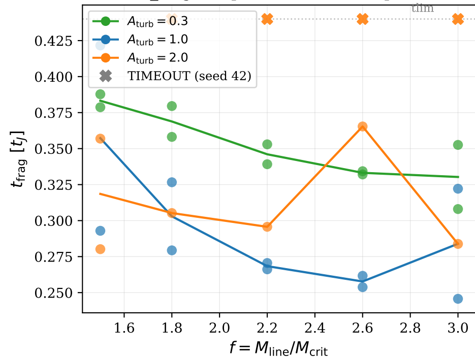
(a) t_{\text{frag}} vs f per turbulence amplitude
