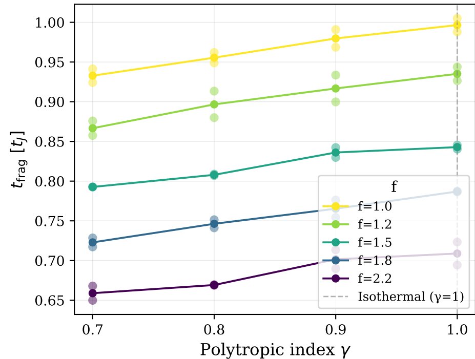
(a) t_{\text{frag}} vs \gamma per mass-ratio f
