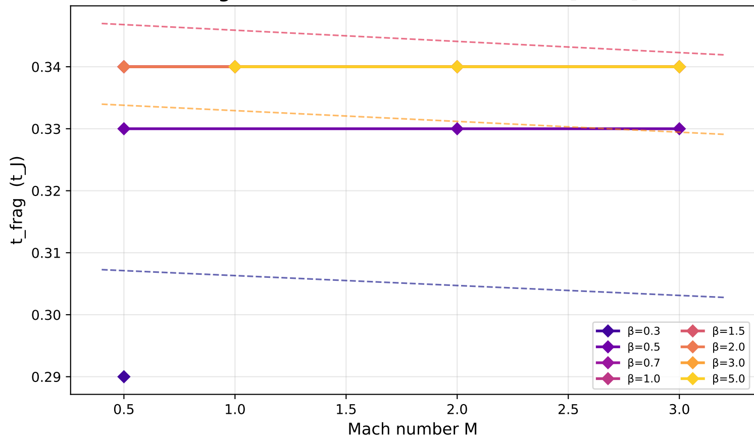
Fragmentation Time vs Mach Number [f=1.5]
