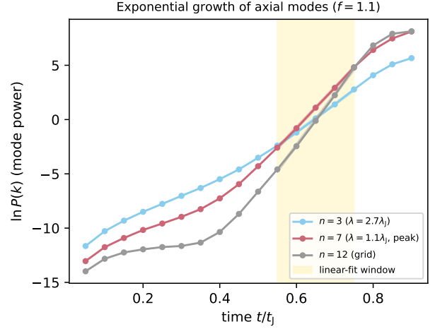
Figure 8. Power in three axial modes versus time for a near-critical filament ( f = 1.1 ). Each grows with an approximately exponential interval (the fit window, shaded) whose slope gives the growth rate; the growth steepens as the filament collapses, so the extracted rate characterises the dominant mode of a dynamically collapsing filament. The peak mode n = 7 grows faster than the long-wavelength n = 3 , giving the sub-classical \lambda_{\text{max}} ; the grid-scale n = 12 is shown for reference.
