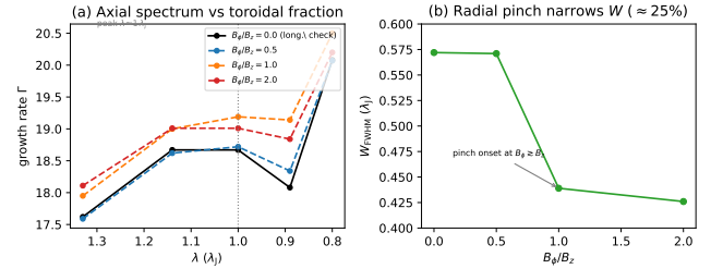
Figure 7. Divergence-free helical-field scan ( B_\phi/B_z = 0 – 2 , 512 \times 128^2 ; Section 4.3). (a) The axial growth-rate spectrum \Gamma(\lambda) in the physical band is invariant to the toroidal fraction ( < 6\% , fit noise), with the plateau peak fixed at \lambda \approx 1 \lambda_J ; B_\phi/B_z = 0 (black) reproduces the pure-longitudinal spectrum, a code check. No excess growth appears at shorter \lambda for any winding. (b) The one systematic effect is a radial pinch : the formation FWHM narrows by \approx 25\% , with onset at B_\phi \gtrsim B_z . The seeded helical field therefore raises \lambda/W by shrinking W , not by shortening \lambda ; the force-balanced Fiege & Pudritz (2000) pinch mode is not tested here.
