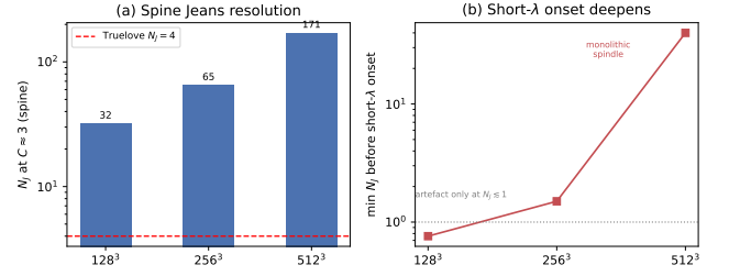
Figure 6. Ideal perpendicular-field refinement ladder ( 128^3 – 512^3 ; Section 4.3). (a) Cells per local Jeans length N_J at the beading-relevant spine contrast C \approx 3 : the collapsing spine is resolved far above the Truelove threshold ( N_J = 4 , dashed) at every resolution. (b) The spurious short- \lambda axial “beading” emerges only once the spine drops below N_J \approx 1 , and refinement pushes that onset to ever-deeper collapse (at 512^3 the filament stays monolithic to N_J \approx 40 at C \approx 30 ) — the short- \lambda onset deepening with resolution being the textbook Truelove under-resolution artefact signature, not a physical fragmentation mode.
