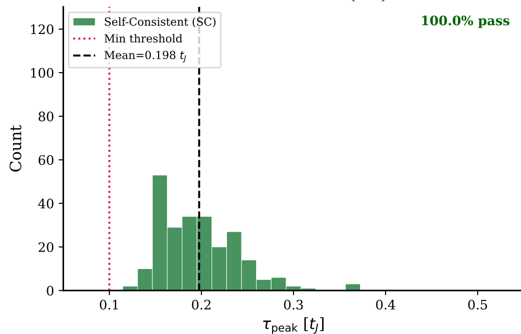
Self-Consistent (SC)
