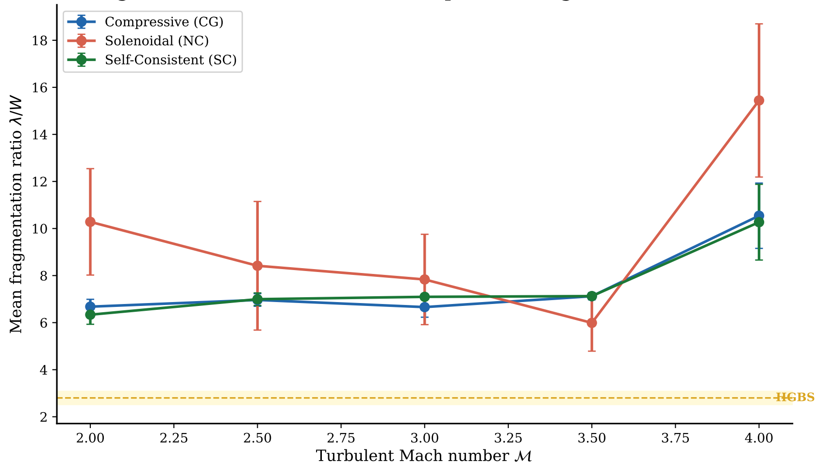
Fragmentation Scale vs Turbulent Amplitude (Longitudinal Field \theta = 0^\circ )
